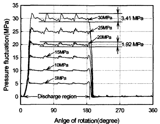
Fig. 6 Pressure variations in cylinder at 1500 rpm (VP2)
