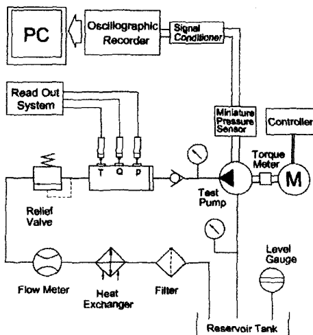
Fig. 4 Hydraulic circuit for test equipment
