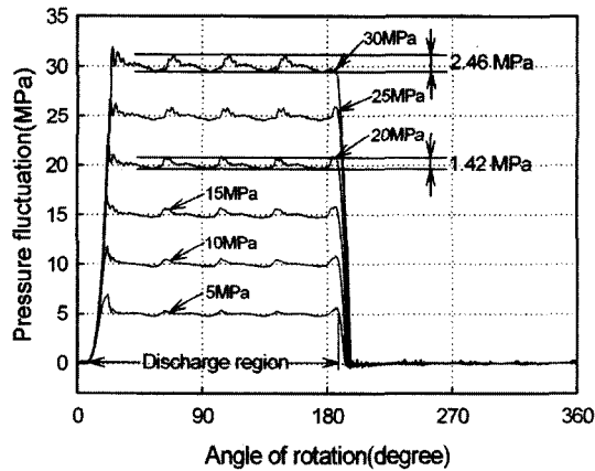
Fig. 7 Pressure variations in cylinder at 1500 rpm (VP3)
