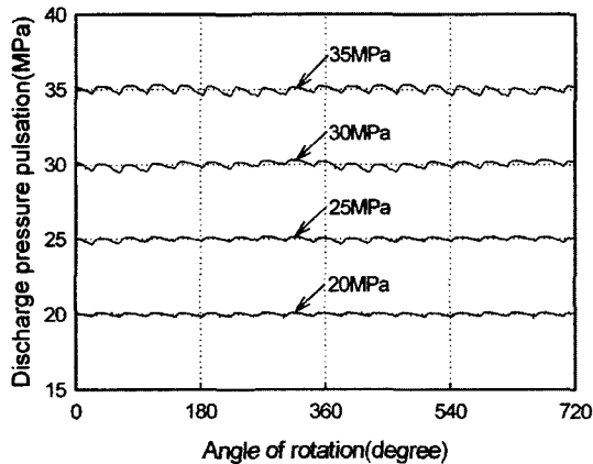
Fig. 11 Pressure pulsations in discharge line (VP2)
