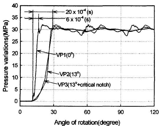
Fig. 8 Comparison of pressure rising slopes at BDC
