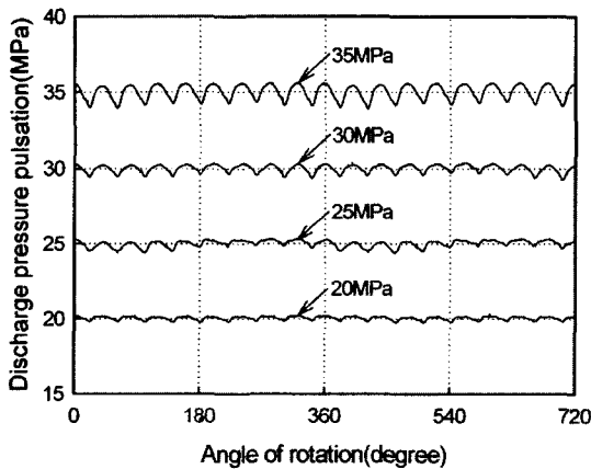
Fig. 10 Pressure pulsations in discharge line (VP1)
