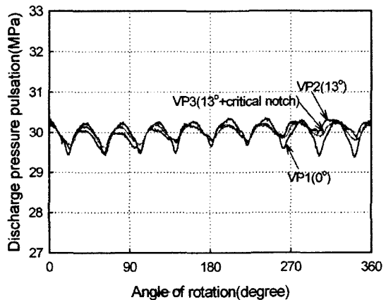
Fig. 13 Comparison of pressure pulsations in discharge line
