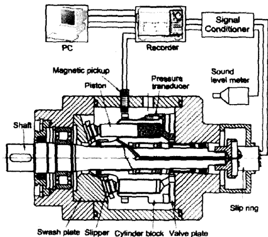
Fig. 2 Schematic diagram of test piston pump
