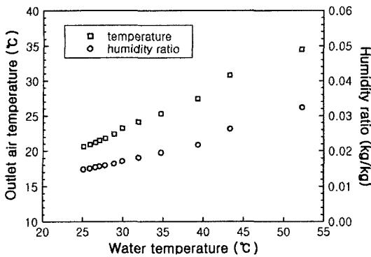
Fig. 12 Variation of outlet air conditions with water temperature for heating
