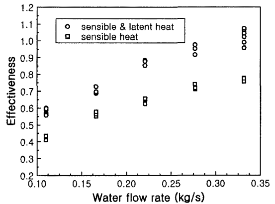
Fig. 8 Effectiveness versus water flow rate for cooling
