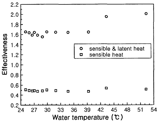
Fig. 13 Effectiveness versus water temperature for heating
