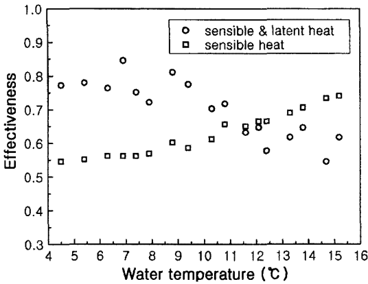
Fig. 9 Effectiveness versus inlet water temperature for cooling
