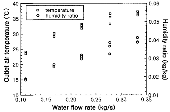
Fig. 10 Variation of outlet air conditions with water flow rate for heating
