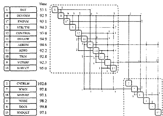
Fig. 6 Result of adaptive parallel decomposition
