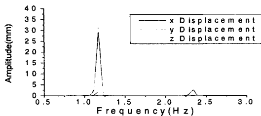
Fig. 13 Natural frequency of the plate
