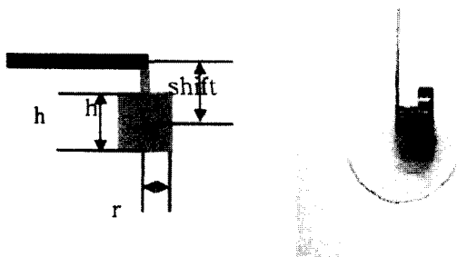
Fig. 4 Attached mass
