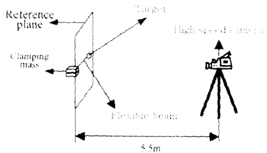
(a) Location of high-speed camera
