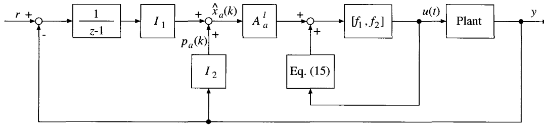
Fig. 2. State-predictive servo system. r is a reference input, u(k) is a manipulated input and y is a controlled output. Eq. (15) is a finite interval summation for state prediction.
