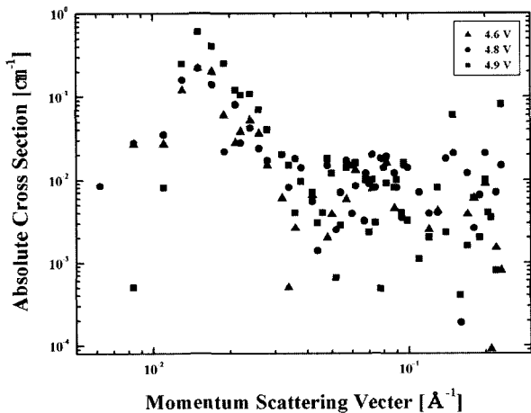
Fig. 3. Distribution of nano-size defects in trivalent chromium layer.
