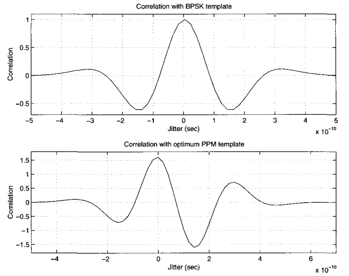
Fig. 2. Correlation functions of the received pulse with the templates used for BPSK and optimum PPM ( \tau = 0.277 ns).
