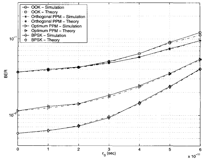
Fig. 5. Effect of the fixed value of timing jitter on the BER performances of different modulation schemes (SNR = 5 dB, T_c = T_h = 0.8 ns, N_s = 1 ).
