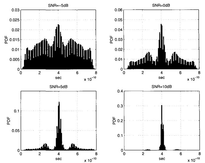
Fig. 10. Probability densities of finger estimation errors ( T_c = T_h = 0.8 ns).
