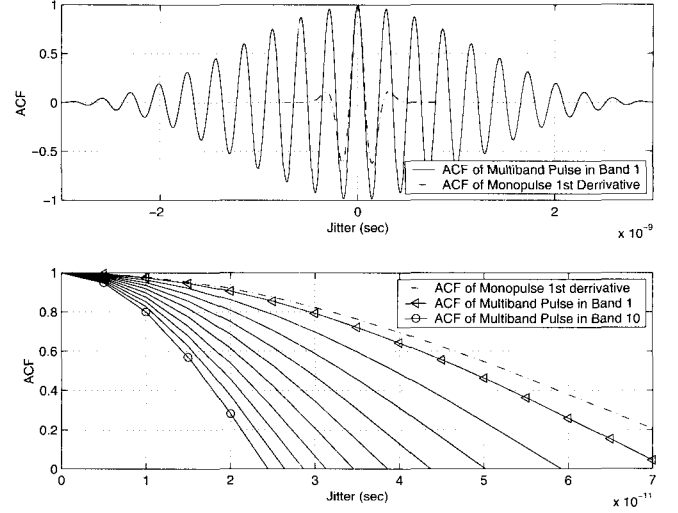
Fig. 13. Comparison of autocorrelation functions of derivative of monocycle vs. pulse used in band 1 of multiband scheme, and comparison of the autocorrelations of the pulses used in all bands.
