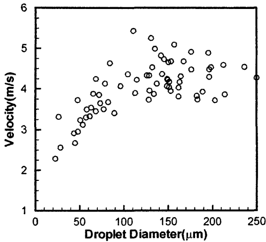
Fig. 10 Distributions of sizes and velocities of droplets
