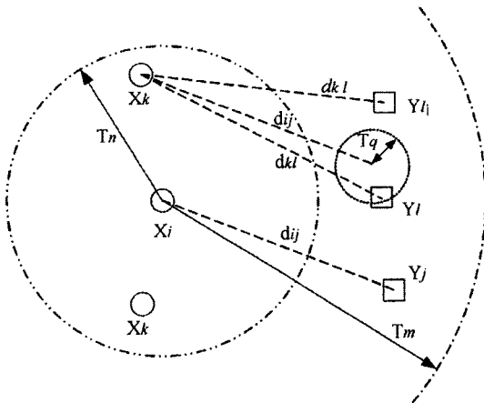
Fig. 8 Particle tracking algorithm by neighboring match probability
