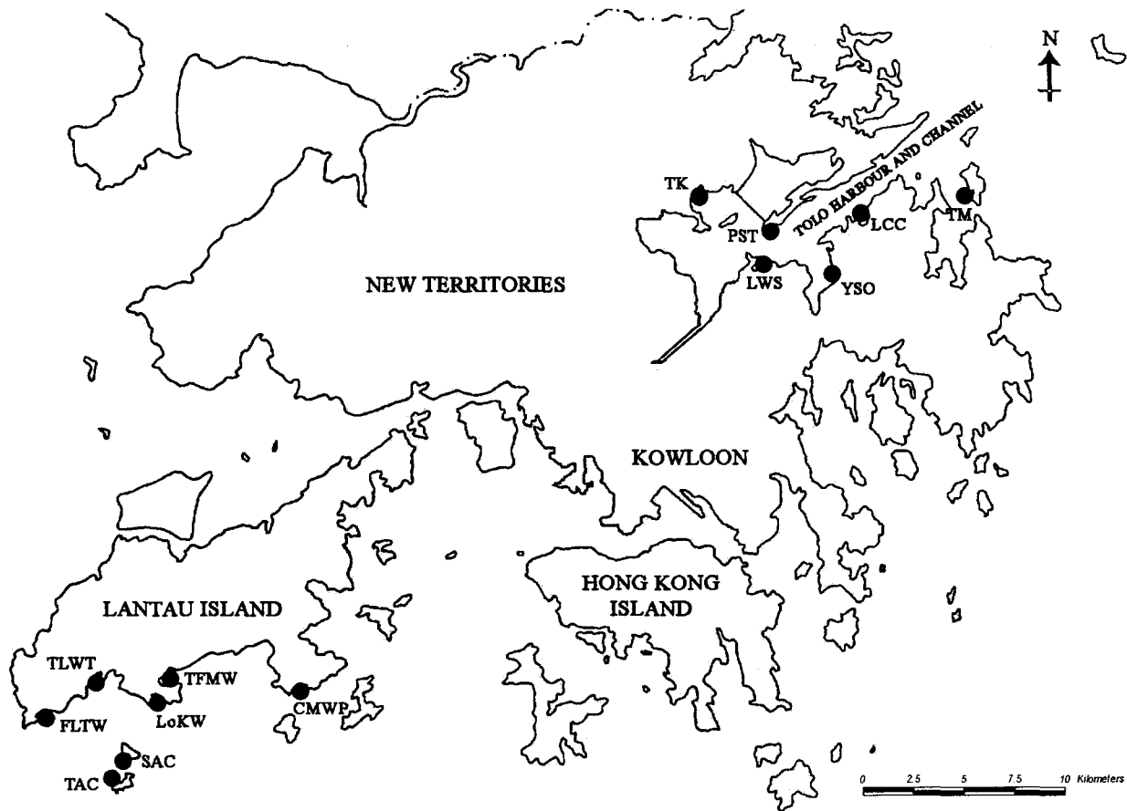
Fig. 1. The soft shores in Hong Kong (LWS - Lok Wo Sha, LCC - Lai Chi Chong, TM - Tap Mun, YSO - Yung Shue O, TK - Ting Kok, PST - Pak Sah Tau, TFMW - Tong Fook Miu Wan, SAC - Siu A Chau, TLWT - Tai Long Wan Tsuen, TAC - Tai A Chau, FLTW - Fan Lau Tung Wan, LoKW - Lo Kei Wan, CMWP - Chi Ma Wan).
