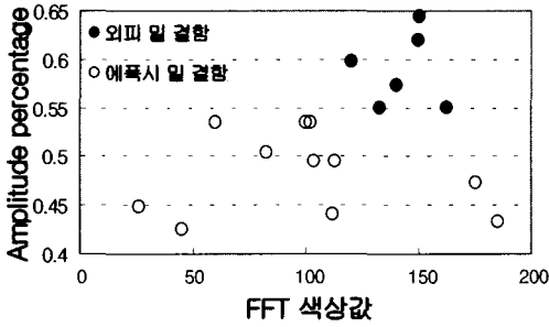
Fig. 8 FFT color value color value versus 20MHz amplitude percentage
