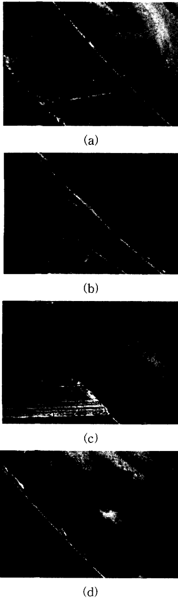
Fig. 6 Microphotographs of the typical defects, (a) missing adhesive under the epoxy, (b) debonding under the epoxy, (c) missing adhesive under the steel sheet, and (d) debonding under the steel sheet
