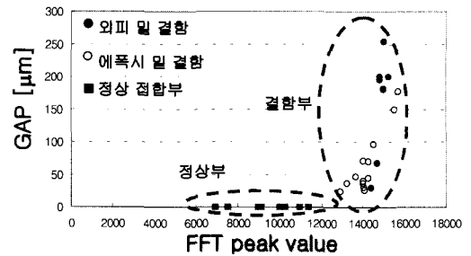
Fig. 7 FFT peak value versus GAP size
