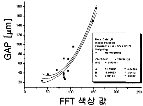
Fig. 10 Regression curve for defects under epoxy
