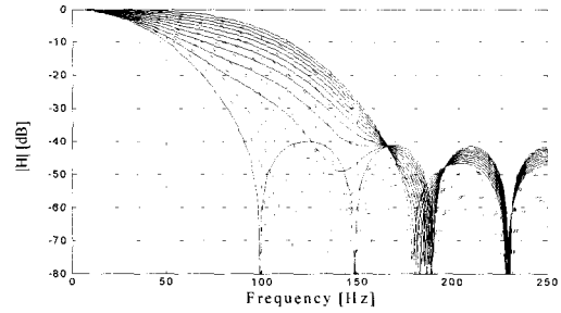
a) N = 12, f_{c0} = 20\text{Hz}, f_{c1} = 100\text{Hz}
