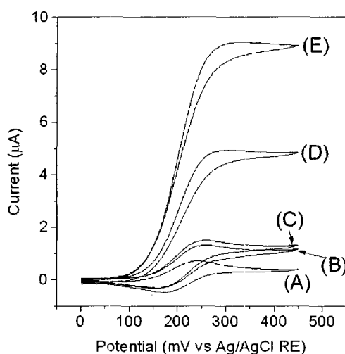
Fig. 3. Cyclic voltammograms of affinity biosensors for avidin by the signaling mode of the diffusible mediator-facilitated electron transfer: (A) background, (B) 0 µg/mL avidin, (C) 100 µg/mL, (D) 1 mg/mL, and (E) 2 mg/mL. Conditions for the electrochemical tests were the same as Fig. 2.
