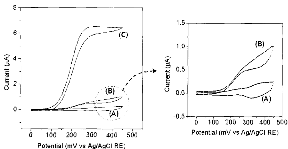
Fig. 2. Voltammetric traces for the affinity biosensor signaling: an avidin-associated surface before (A) and after (B) the b-GOx treatment and bioelectrocatalysis. Trace (C) was registered after the addition of a 0.1 mM ferrocene methanol mediator in the electrolyte. Measurements were performed in a 0.1 M phosphate buffer (pH 7.0) under the potential sweep rate of 5 mV/s. A magnified view of the voltammograms (A) and (B) is presented for clarity on the right.
