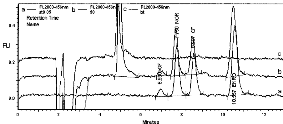
Fig. 3. Chromatograms of four fluoroquinolone. a; 50 ng/ml of four fluoroquinolone standards, b; chicken muscle fortified with 50 ng/g of four fluoroquinolones, c; blank chicken muscle.
