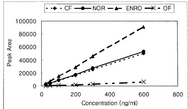
Fig. 2. Standard calibration curves of four fluoroquinolones ( \gamma^2 > 0.999 ). OF: Ofloxacin, NOR: Norfloxacin, CF: Ciprofloxacin, ENRO: Enrofloxacin.
