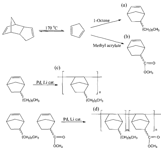
Scheme 1. Synthetic routes to (a) Hexylnorbomene, (b) Methyl ester norbornene, (c) poly(HNB) and (d) poly(HNB-co-MES-NB).
