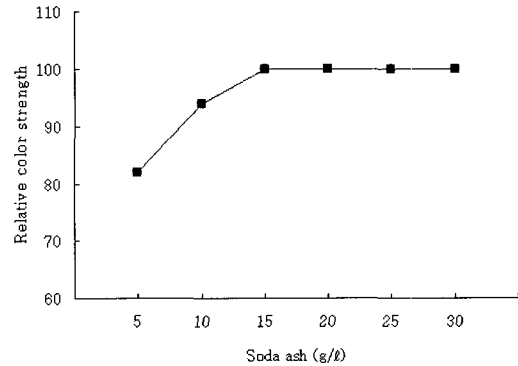
Fig. 11. Alkali sensitivity of antibiotic red reactive dye.
