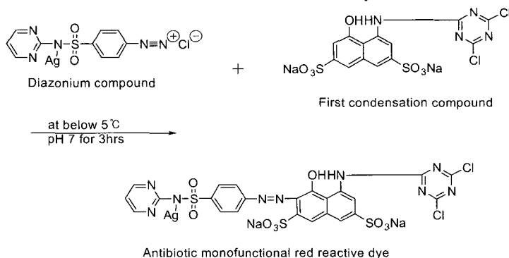
Scheme 6. Coupling reaction between diazonium compound of silver sulfadiazine and first condensation compound.
