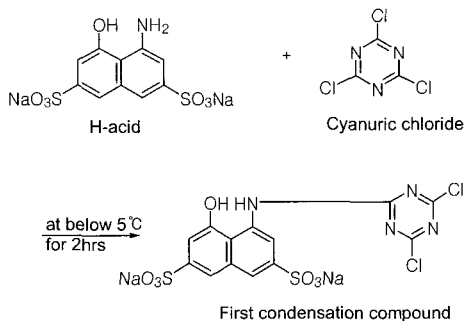
Scheme 5. The first condensation reaction between H-acid and cyanuric chloride.
