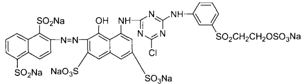
Scheme 8. Structure of C. I. Reactive Red 195.
