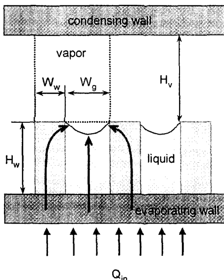
Fig. 2 Cross-sectional view of vapor chamber heat spreader
