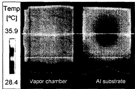
(b) For the forced convection heat transfer with air blowing of 3 m/s
