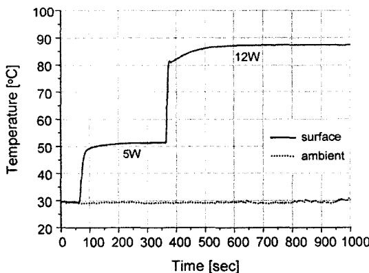
Fig. 8 Transient temperature response by varying heat inputs
