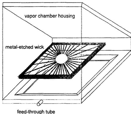
Fig. 4 Configuration of the vapor chamber heat spreader
