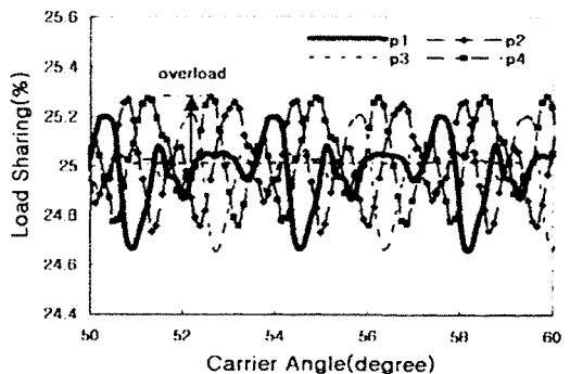
Fig. 3 Bearing forces and planet load sharing under normal conditions with four planets
