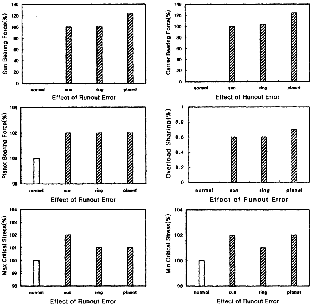
Fig. 15 Trends in the maximum bearing forces and critical stresses due to the effect of runout error with three planets, error = 25 \mu m
