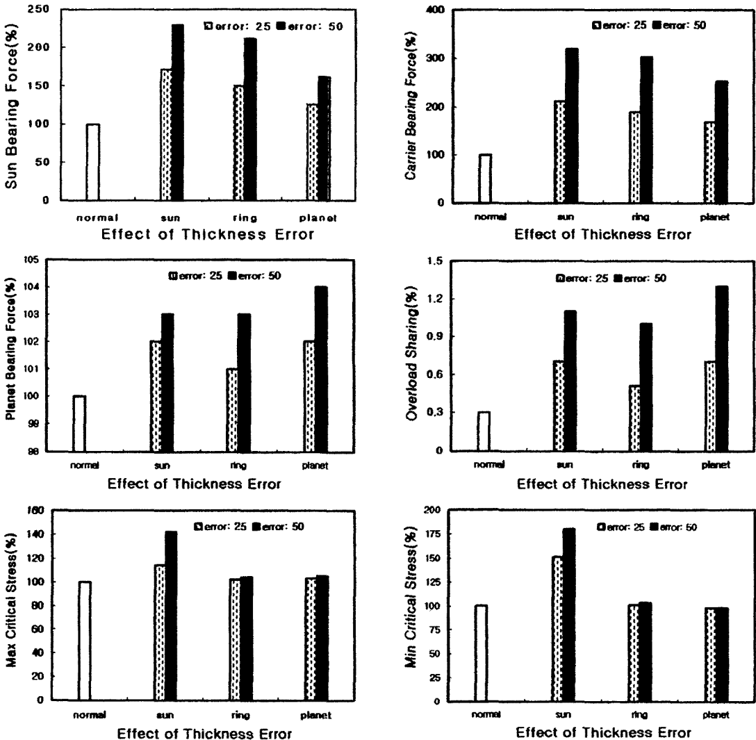
Fig. 18 Maximum bearing forces and critical stresses caused by tooth thickness error with four planets
