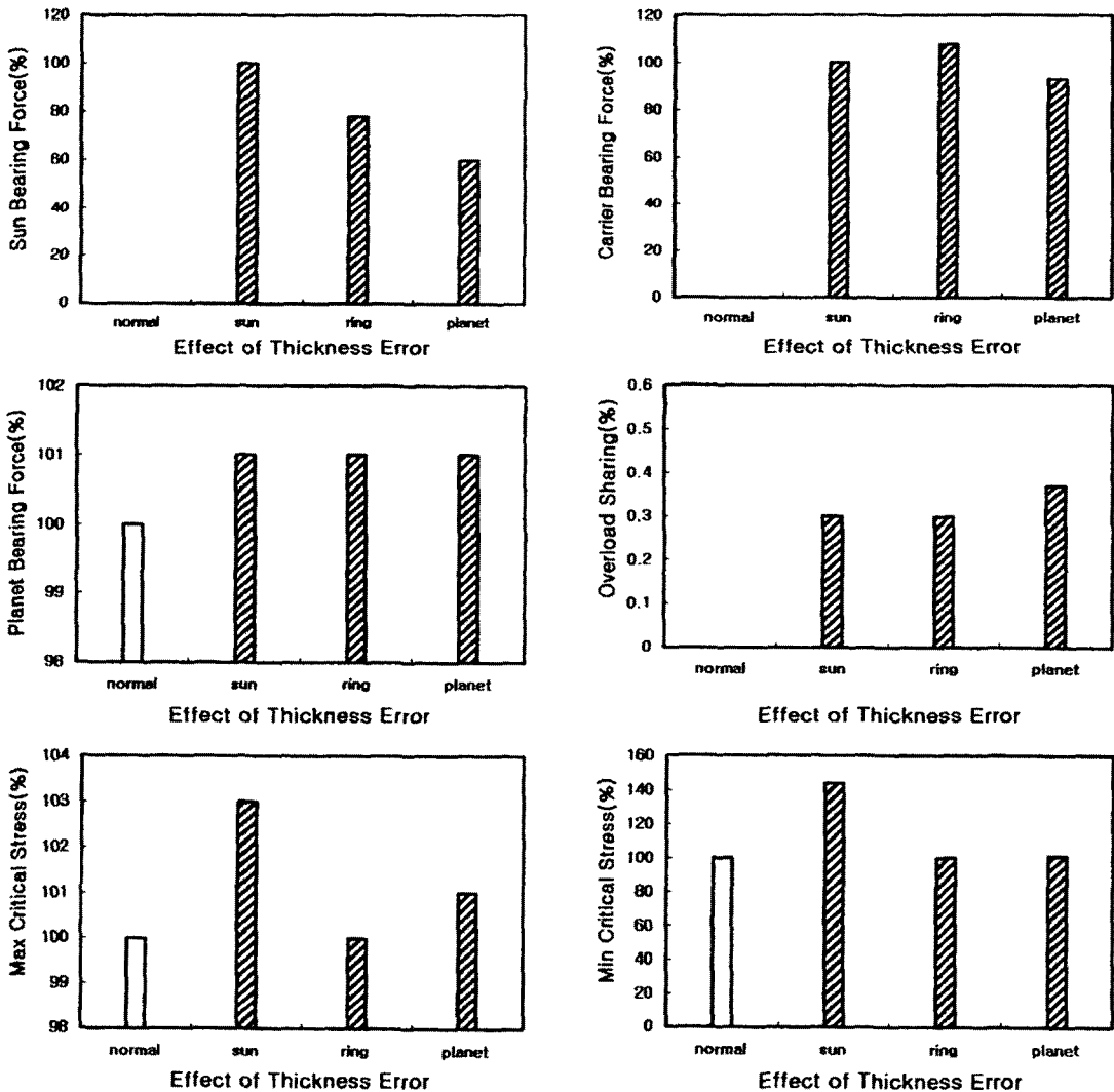
Fig. 19 Maximum bearing forces and critical stresses caused by a 25- \mu m tooth thickness error with three planets
