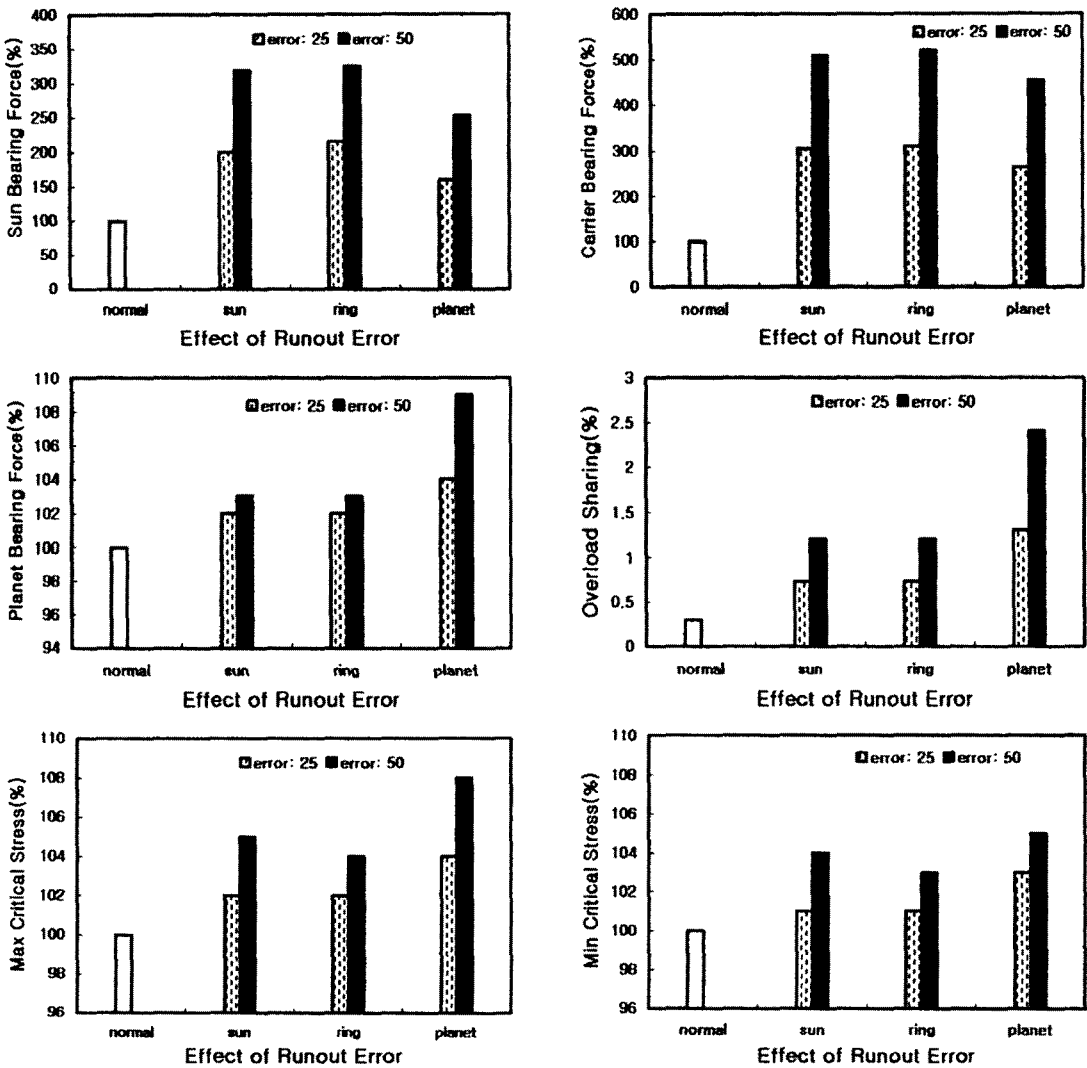
Fig. 14 Trends in the maximum bearing forces and critical stresses due to the effect of runout error with four planets
