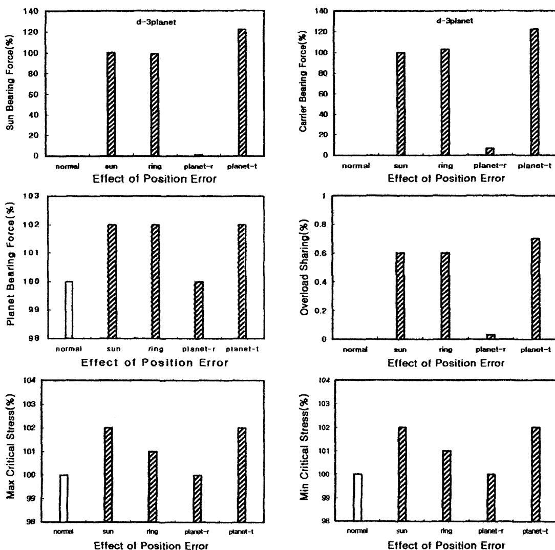
Fig. 10 Trends in the maximum bearing forces and critical stresses due to the effects of a position error with three planets, error=25 \mu m
