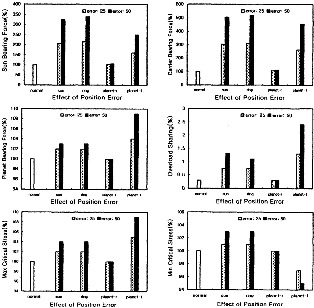
Fig. 9 Trends in the maximum bearing forces and critical stresses due to the effects of a position error with four planets
