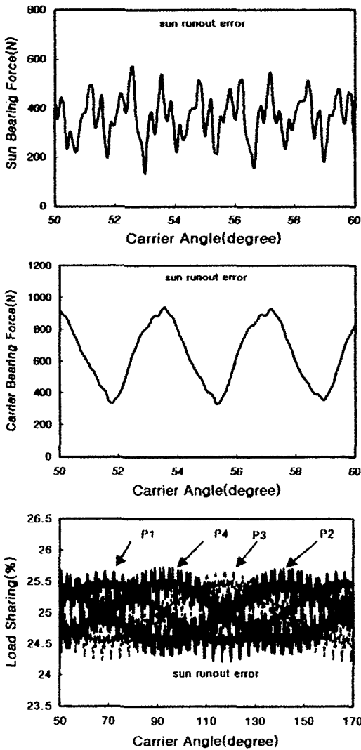
Fig. 11 Sun and carrier bearing forces and planet load sharing with a sun gear runout error of 25 \mu\text{m} with four planets
