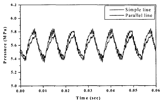
Fig. 8 Comparison of simulated results in inlet pressure between simple and parallel line with rotational speed 1000rpm
