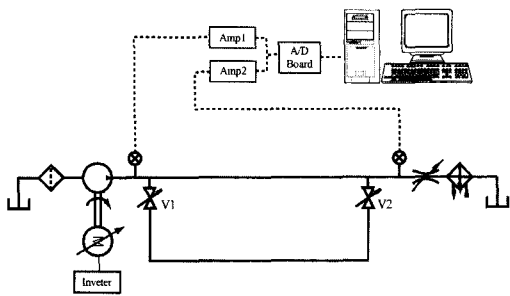
Fig. 5 Schematic diagram of the experiment
