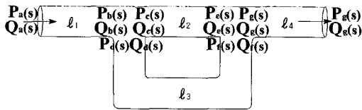
Fig. 2 Hydraulic pipeline with a parallel line
