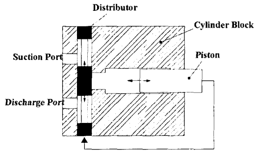
Fig. 3 Operating principle of a piston in a bent axis piston pump
