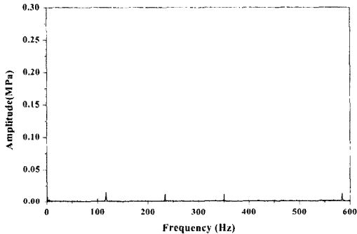
Fig. 13 Frequency analysis of outlet pressure in parallel line
