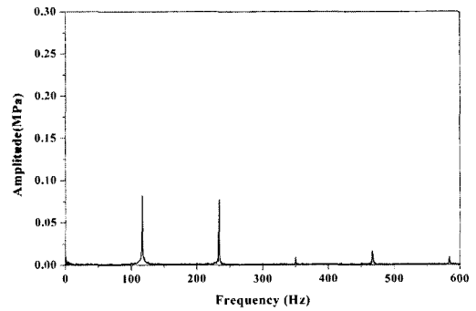
Fig. 9 Frequency analysis of inlet pressure in parallel line
