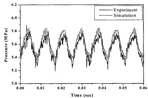
Fig. 6 Comparison of discharge pressure between simulation and experiment with rotational speed 1000rpm
