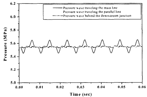
Fig. 16 Effect of phase interference at downstream junction
