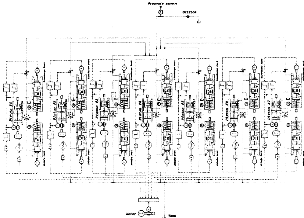
Fig. 4 Modeling for a bent-axis piston pump
