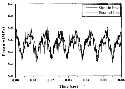
Fig. 7 Comparison of experimental results in inlet pressure between simple line and parallel line with rotational speed 1000rpm
