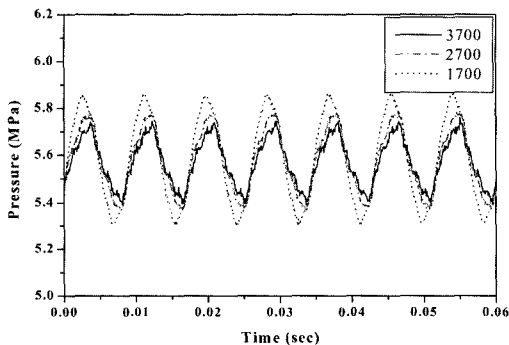
Fig. 14 Simulated results in inlet pressure of parallel line by the change of length of parallel line
