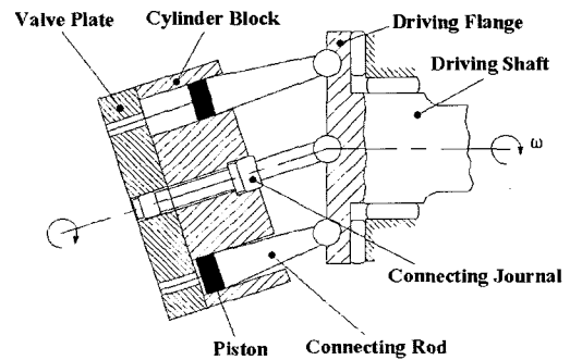
Fig. 1 Configuration of a bent-axis piston pump
