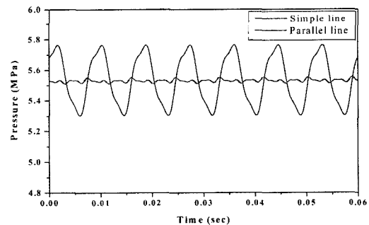
Fig. 11 Comparison of simulated results in outlet pressure between simple line and parallel line with rotational speed 1000rpm
