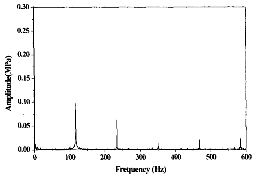
Fig. 12 Frequency analysis of outlet pressure in simple line
