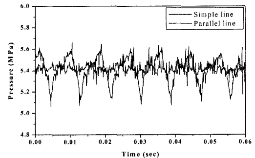
Fig. 10 Comparison of experimental results in outlet pressure between simple line and parallel line with rotational speed 1000rpm
