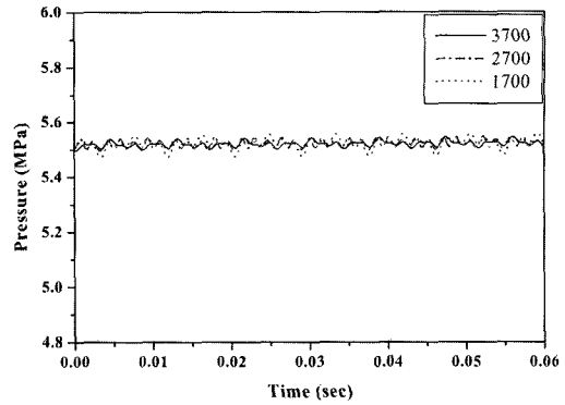
Fig. 15 Simulated results in outlet pressure of parallel line by the change of length of parallel line
