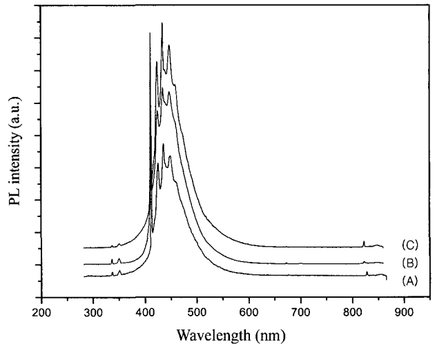
Fig. 3. Low-temperature photoluminescence spectra in the region from 325 to 850 nm are shown for HPHT treated diamonds : (A) F color grade, (B) D color grade, (C) G color grade.
