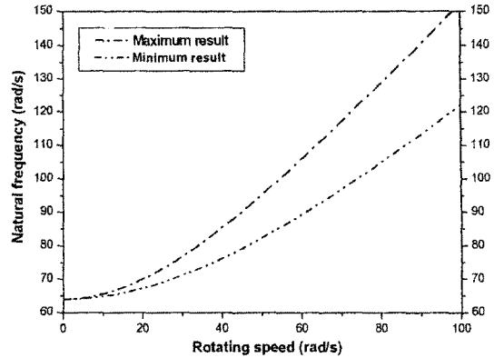
Fig. 6 Band of the fundamental natural frequency versus rotating speed
