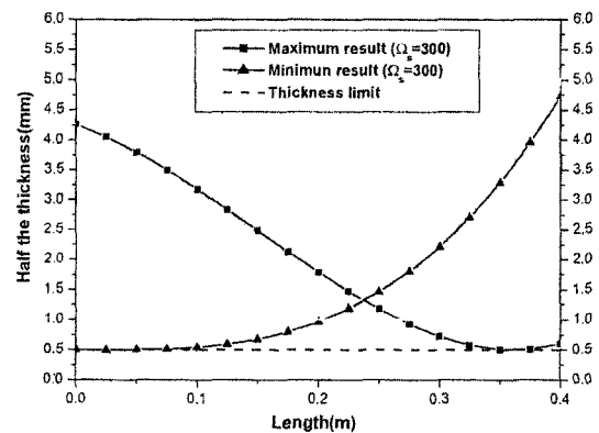
Fig. 4 Half the thickness shapes which maximize and minimize the fundamental natural frequency
