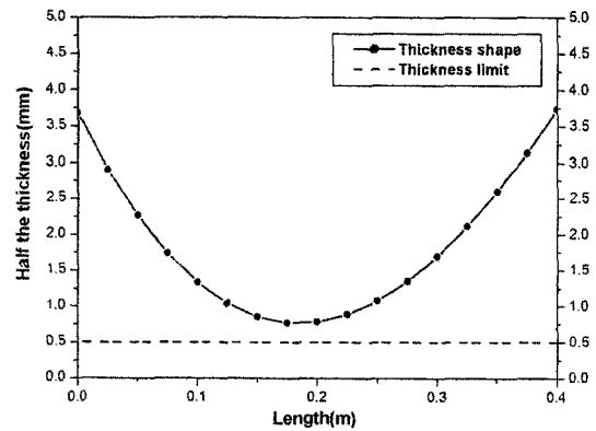
Fig. 12 Half the thickness shape of the beam which satisfies the specified first natural frequency
