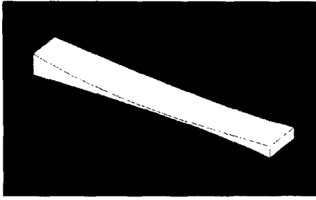
Fig. 9 Beam shape which maximizes fundamental natural frequency
