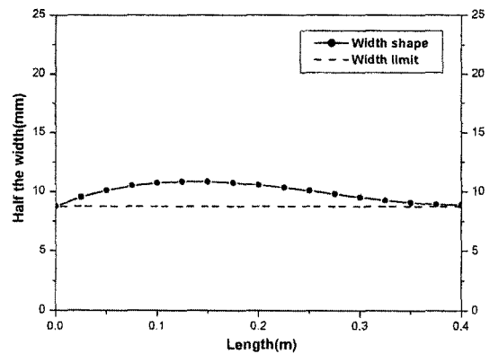
Fig. 13 Half the width shape of the beam which satisfies the specified first natural frequency
