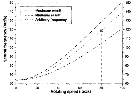
Fig. 11 Specified fundamental natural frequency locus along with the maximum and the minimum loci
