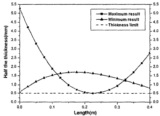
Fig. 7 Half the thickness shapes which maximize and minimize the fundamental natural frequency
