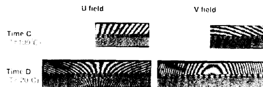
Fig. 7 U and V displacement field patterns of the large ceramic BGA package assembly (CBGA 19)
