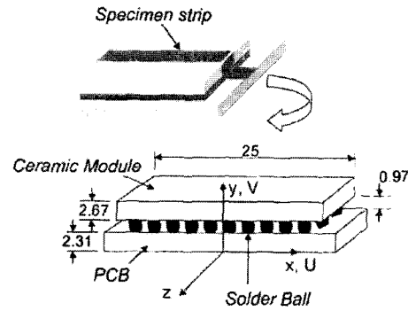
Fig. 4 Schematic diagram of the ceramic BGA package assembly geometry with relevant dimensions (mm)
