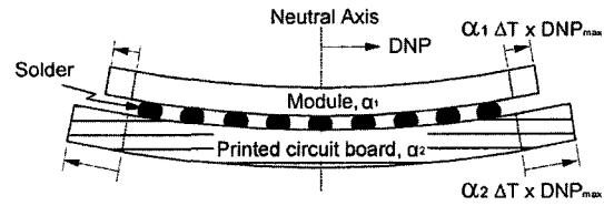
Fig. 1 Global deformation of BGA package assembly due to temperature change
