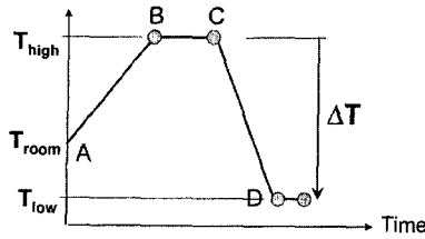
Fig. 5 Temperature profile used in the experiment of the ceramic BGA package assembly
