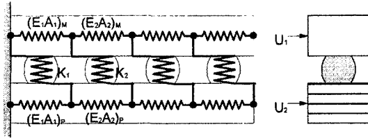
Fig. 2 Network of compact spring model for the determination of thermal displacement of package assembly
