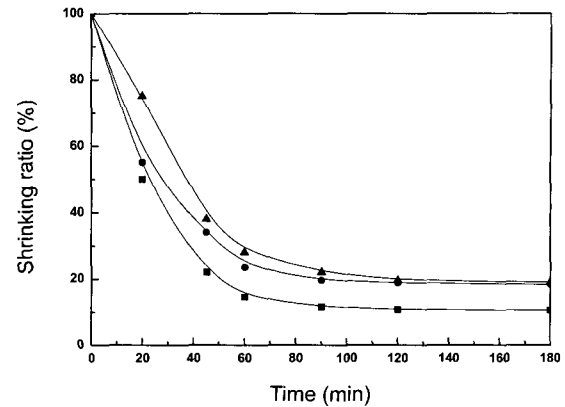
Figure 3. Deswelling kinetics of PNIPAAm gel in 10 mmol Tris-HCl buffered solution as a function of time at various concentrations: 1% w/v (■), 2% w/v (●), and 4% w/v (▲). The temperature was 37 °C.
