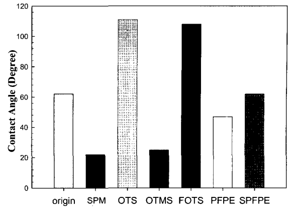
Figure 3. Water contact angle of various SAMs coated silicon surface.
