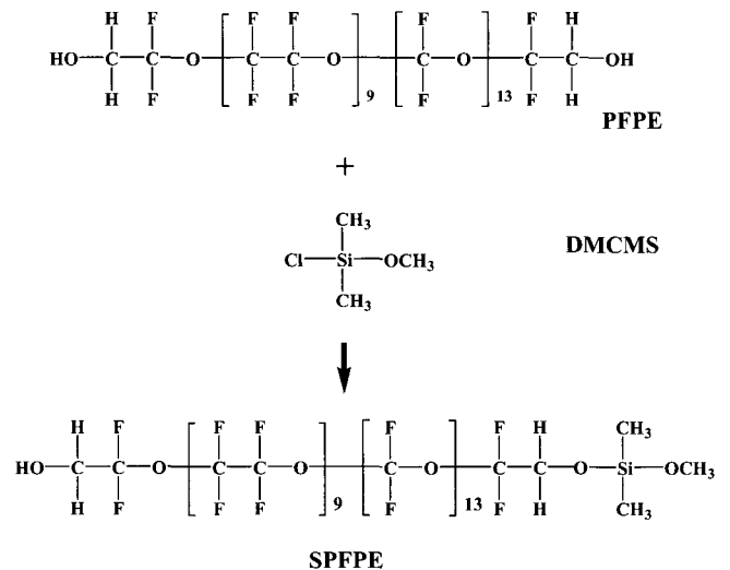
Figure 1. Modification scheme of silane modified PFPE.
