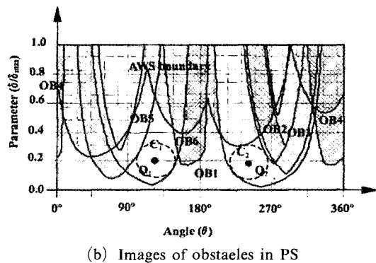
Fig. 11 Simulation of CM (case 1) — robot workspace and images of each obstacle in PS
