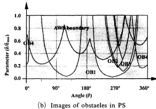
Fig. 12 Simulation of CM (case 2) — robot workspace and images of each obstacle in PS
