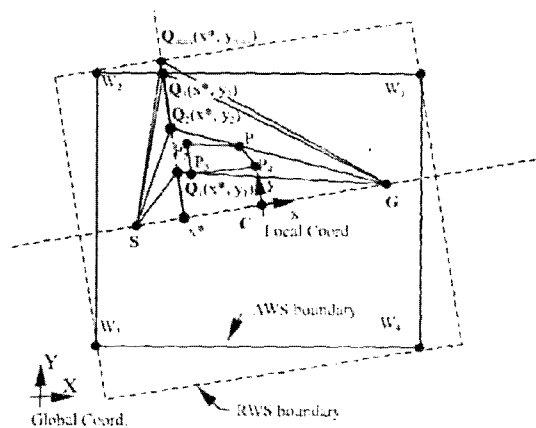
Fig. 14 Cartesian coordinate of intermediate connection point and RWS GM
