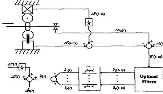
Fig. 2 Eccentricity estimator and output thickness prediction
