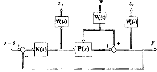
Fig. 3 Feedback control system for the generalized plant with weighting functions
