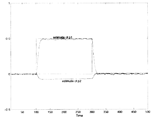
Fig. 4. Result of friedland's approach.
