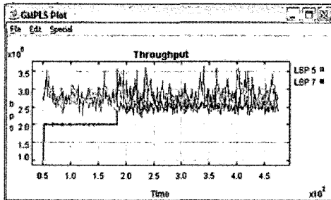
Fig. 6. Throughput LSP 5 and LSP 7
