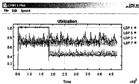
Fig. 7. Utilization of Four LSPs
