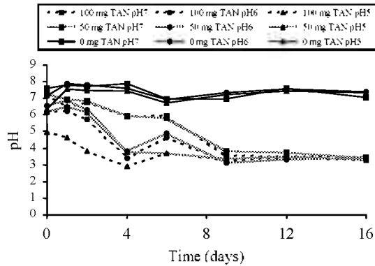
Figure 2. Change in pH over time in pots containing duckweed, as influenced by initial pH and total ammonia nitrogen (TAN) concentration (mg/l)
