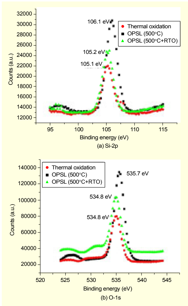
Fig. 7. XPS analysis of an OPSSL.
