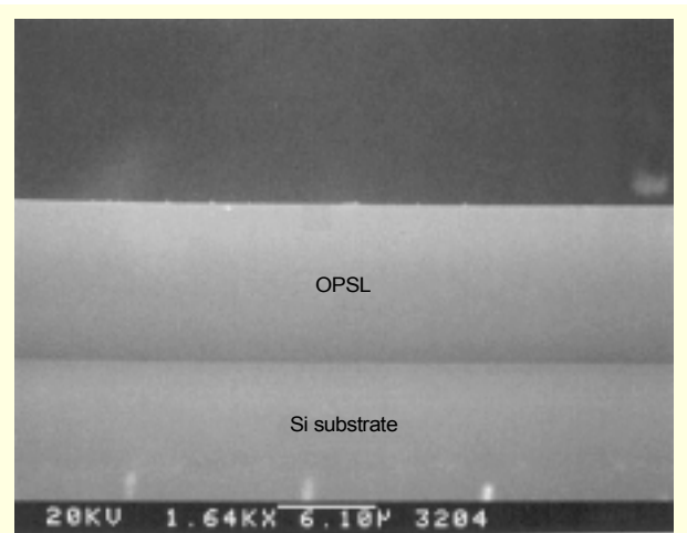
Fig. 2. Cross-sectional SEM image of OPSL surface with newly developed oxidation process.
