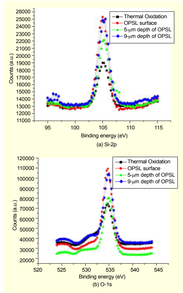
Fig. 8. XPS analysis of an OPSSL with respect to depth.
