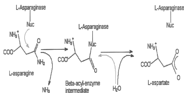
Fig. 1. Schematic illustration of the reaction mechanism of L-asparaginase. (Hill et al. , 1967)
