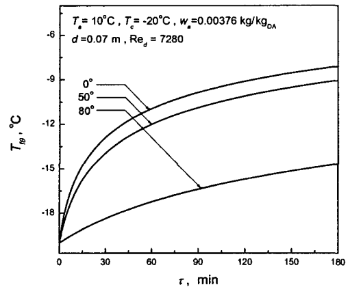
(b) Frost surface temperature
