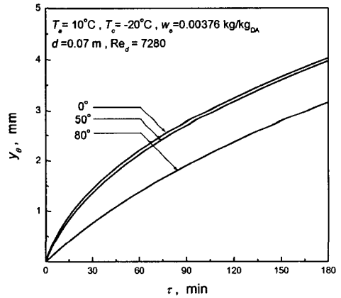
(a) Frost thickness
