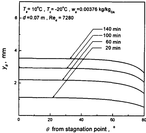
Fig. 5 Variations of the frost thickness along the angular coordinate for different times
