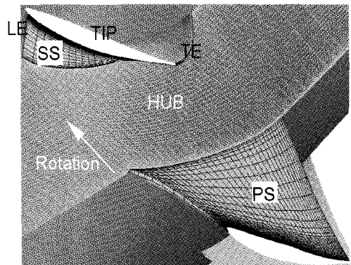
(b) Perspective view (main grid)
