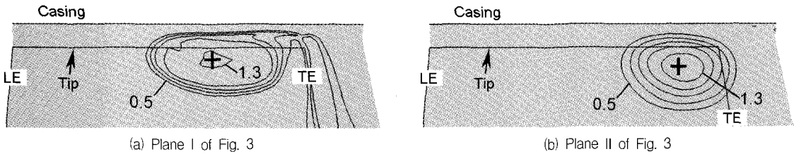
Fig. 13 Distribution of total pressure loss on meridional planes (TC = 4.5 mm, interval of contour lines = 0.2)
