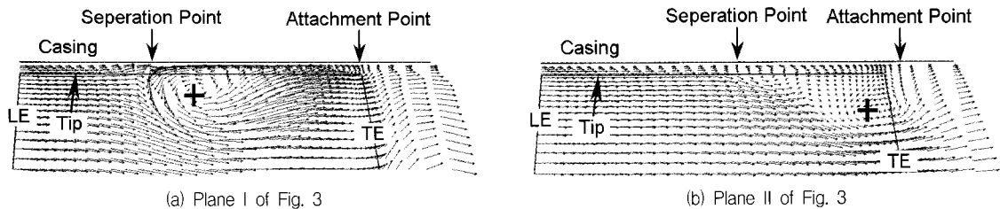
Fig. 8 Distribution of meridional velocity vectors on meridional planes (TC = 2 mm)
