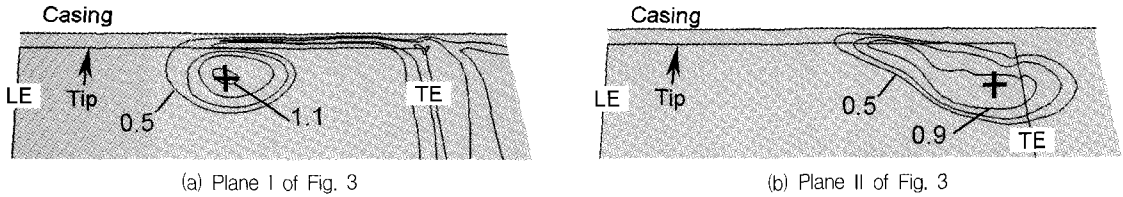
Fig. 12 Distribution of total pressure loss on meridional planes (TC = 2 mm, interval of contour lines = 0.2)
