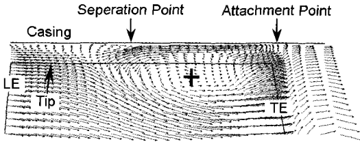
(a) Plane I of Fig. 3
