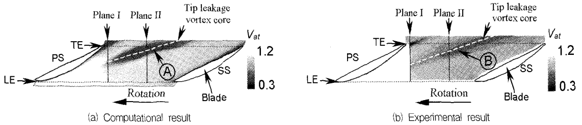
Fig. 3 Distribution of relative velocity on the plane of 99 percent blade height (TC = 2 mm)
