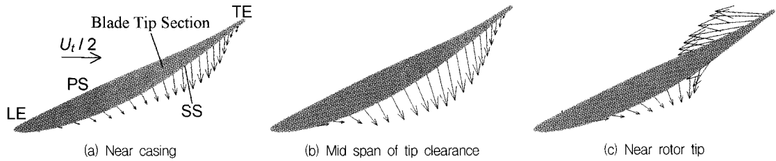
Fig. 7 Distributions of leakage velocity vectors in tip clearance region (TC = 4.5 mm)
