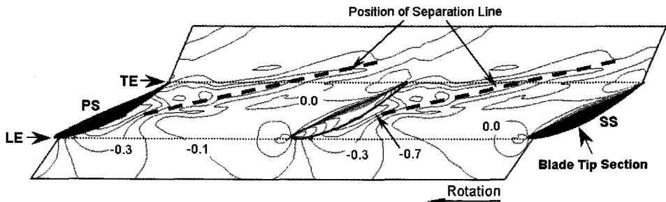
(b) Pressure distribution on casing wall (interval of contour lines = 0.1)
