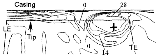
(b) Plane II of Fig. 3
