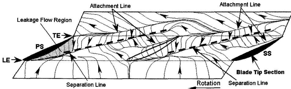
(a) Limiting streamlines on casing wall
