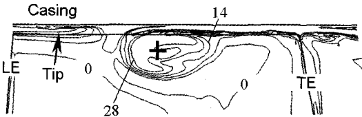
(a) Plane I of Fig. 3
