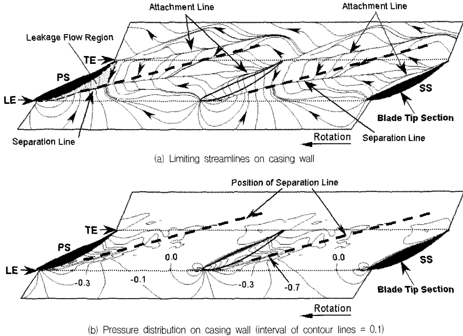
Fig. 4 Limiting streamlines and pressure distribution on casing wall (TC = 2 mm)
