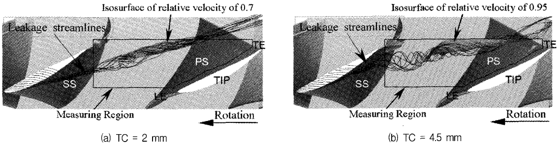
Fig. 2 Leakage streamlines (computational result) and isosurface of relative velocity (experimental result) for two tip clearances (TCs)
