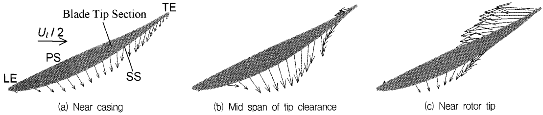
Fig. 6 Distributions of leakage velocity vectors in tip clearance region (TC = 2 mm)
