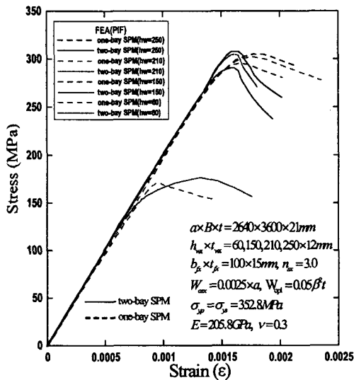
Fig.11 A comparison stress with strain curves of SPM model under axial compression according to the web height and analysis range
