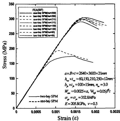
Fig.10 A comparison stress with strain curves of SPM model under axial compression according to the web height and analysis range
