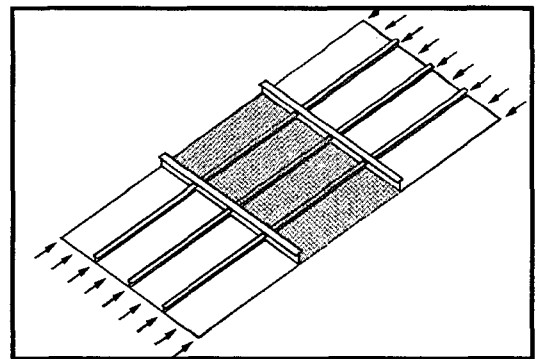
Fig.5 FEA model - One bay SPM (Stiffener Panel Combination)
