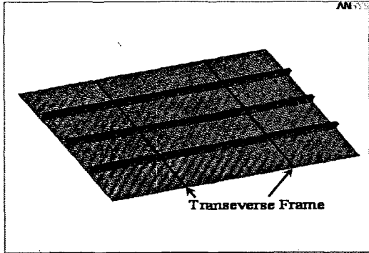
Fig. 7 Idealization of FEA model - Two bay SPM (by ANSYS)
