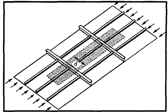
Fig.4 FEA model - Two bay PSC (Plate-Stiffener Combination)
