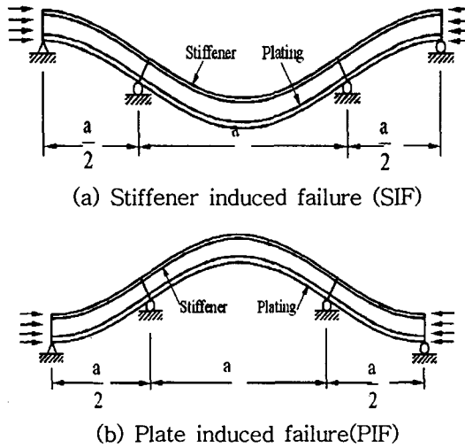
Fig. 2 A Schematic representation of PIF and SIF patterns in the two bay model
