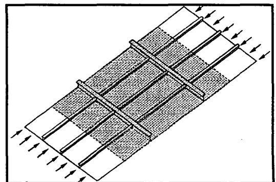
Fig.6 FEA model - Two bay SPM (Stiffener Panel Combination)
