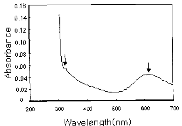
Fig. 4. Absorbance spectrum of laccase from T. hirsuta S1 (0.3 mg in 100 mM sodium acetate, pH 5.0) at 25°C. The arrows indicate the characteristic absorbance peak corresponding to type I (ca. 610 nm) and III (ca. 330 nm).
