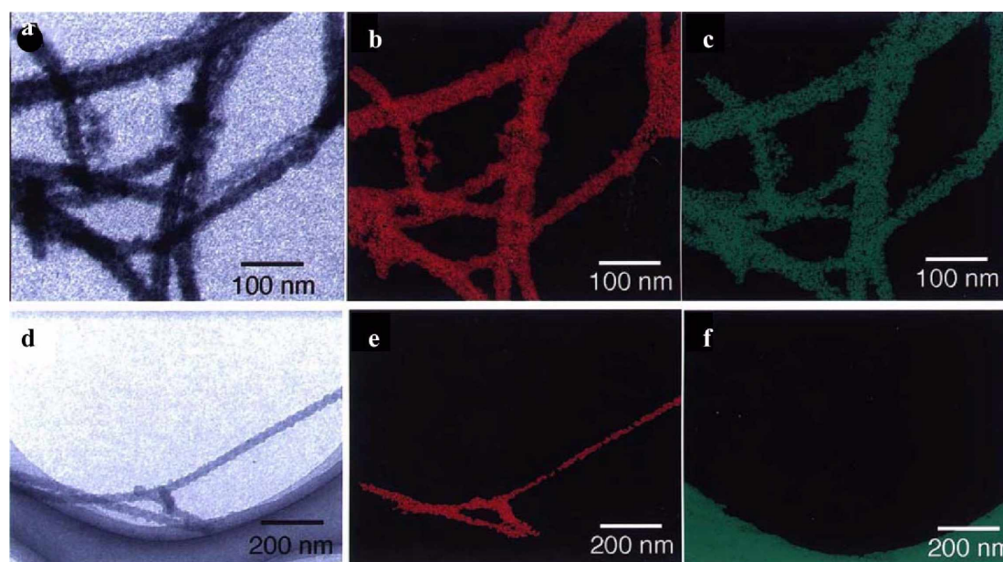
Figure 4. TEM images with electron energy-loss spectroscopy (EELS) of the double-helical silica nanotube obtained from the mixed gel of 1 and 2 (1 : 1 w/w). (a) zero-loss image, (b) silicon component and (c) carbon component before calcination. (d) zero-loss image, (e) silicon component and (f) carbon component after calcination.
