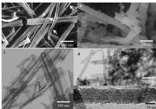
Figure 3. FE-SEM images of the silica nanotube obtained from the mixed gel of (a) 2+5 and (b) 3+4 (1 : 1 w/w) after calcinations. EF-TEM images of the silica nanotubes (c) 2+5 and (d and e) 3+4 (1 : 1 w/w) after calcinations.
