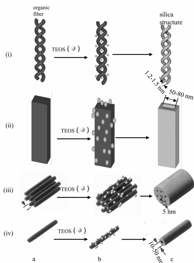
Figure 5. Schematic representation for the creation of various silica structures from the organogel state of 1 (i), 2 (ii) and 3 (iii and iv) by sol-gel polymerization: (a) gelators; (b) sol-gel polymerization of TEOS and adsorption onto the gelators and (c) double-helical structure (i), ribbon structure (ii), single and lotus-like structure (iii and iv) of the silica materials formed after calcination (SEM and TEM pictures in Figs. 1, 2 and 3 were taken at this stage).
