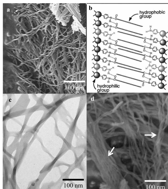
Figure 1. (a) FE-SEM image of the xerogel prepared from the mixed gel of 1 and 4 ( 1 : 4 = 1 : 1 w/w) in water-methanol (10 : 1 v/v). (b) A possible self-assembling model in the bilayered chiral fiber from the mixed gel of 1 and 4 . EF-TEM images of the xerogel prepared from the mixed gel of (c) 2 and 5 ( 2 : 5 = 1 : 1 w/w) and (d) 3 and 4 ( 3 : 4 = 1 : 1 w/w).
