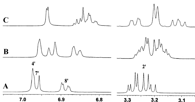
Figure 3. Partial ^1\text{H} NMR spectra of 10 mM nonracemic NA [ R(-)/S(-) = 1 : 2 ] enantiomers in the absence (A) or presence of 10 mM \beta -CD (B) and 10 mM CM- \beta -CD (C).
