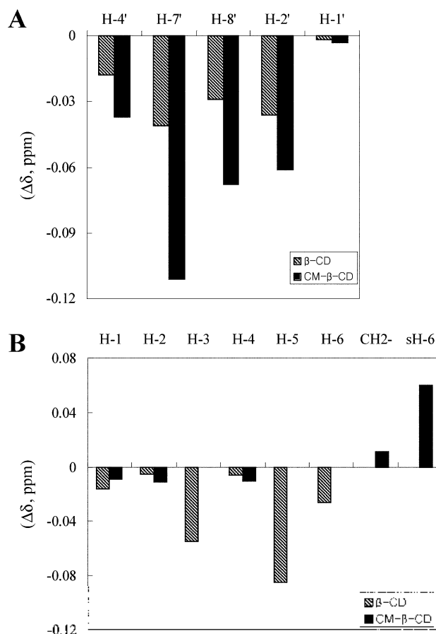
Figure 2. Changes ( \Delta\delta = \delta_{complex} - \delta_{free} , ppm) in the 1 H NMR chemical shifts of NA (A) \beta -CD and CM- \beta -CD (B) upon the complexation. Chemical shifts of the H-3, H-5 and H-6 protons of CM- \beta -CD were not measured due to overlap.
