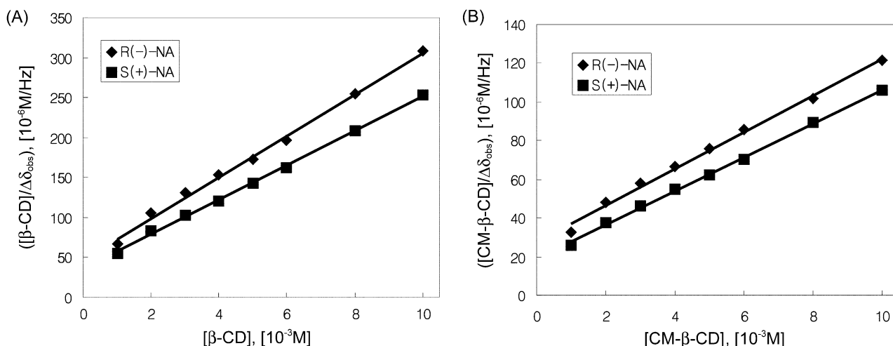
Figure 6. Scott's plots for the complexes of NA enantiomers with \beta -CD (A) or CM- \beta -CD (B).
