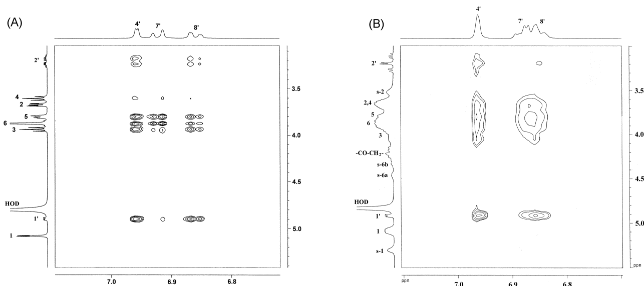
Figure 7. ROESY spectra of the complexes of equimolar racemic NA with 10 mM \beta -CD (A) or CM- \beta -CD (B) in D_2O at 25 °C. (s-1, s-2, s-6a and s-6b: the protons of CM- \beta -CD substituted with carboxymethyl group. -CO-CH 2 -: methylene protons of carboxymethyl group).
