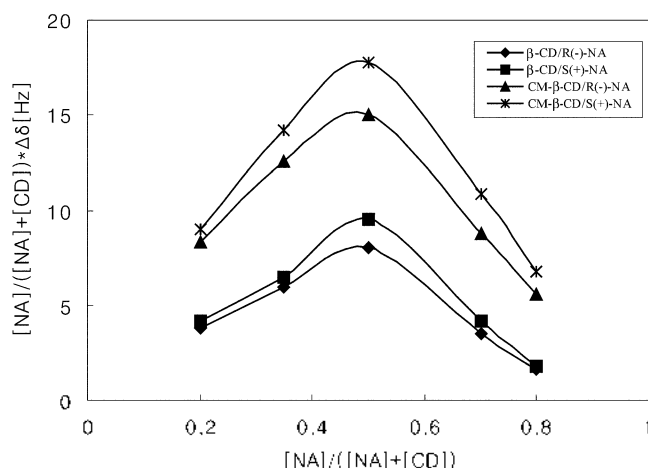
Figure 5. Job plots for the complexes of racemic NA with \beta -CD or CM- \beta -CD.
