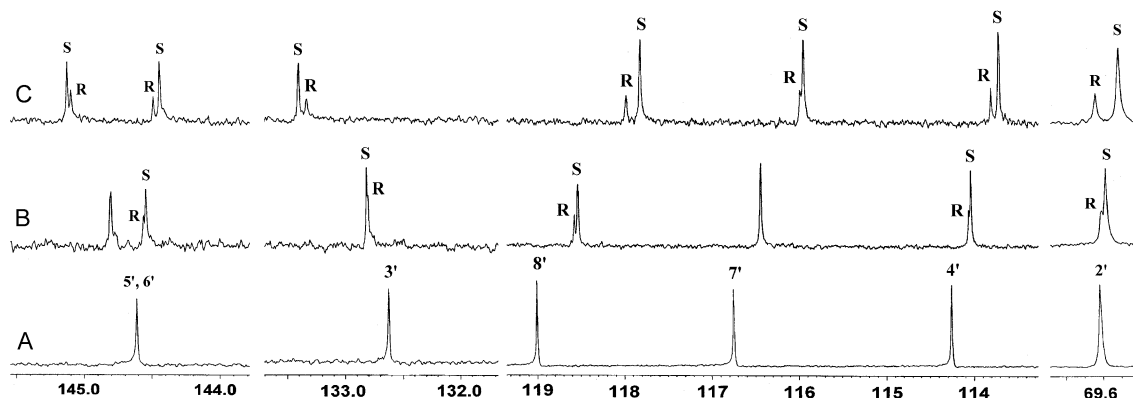
Figure 4. Partial ^{13}\text{C} NMR spectra of 10 mM nonracemic NA [ R(-)/S(-) = 1 : 2 ] enantiomers in the absence (A) or presence of 10 mM \beta -CD (B) and 10 mM CM- \beta -CD (C).
