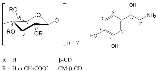
Figure 1. Chemical structures of \beta -CD, CM- \beta -CD (left) and NA (right).
