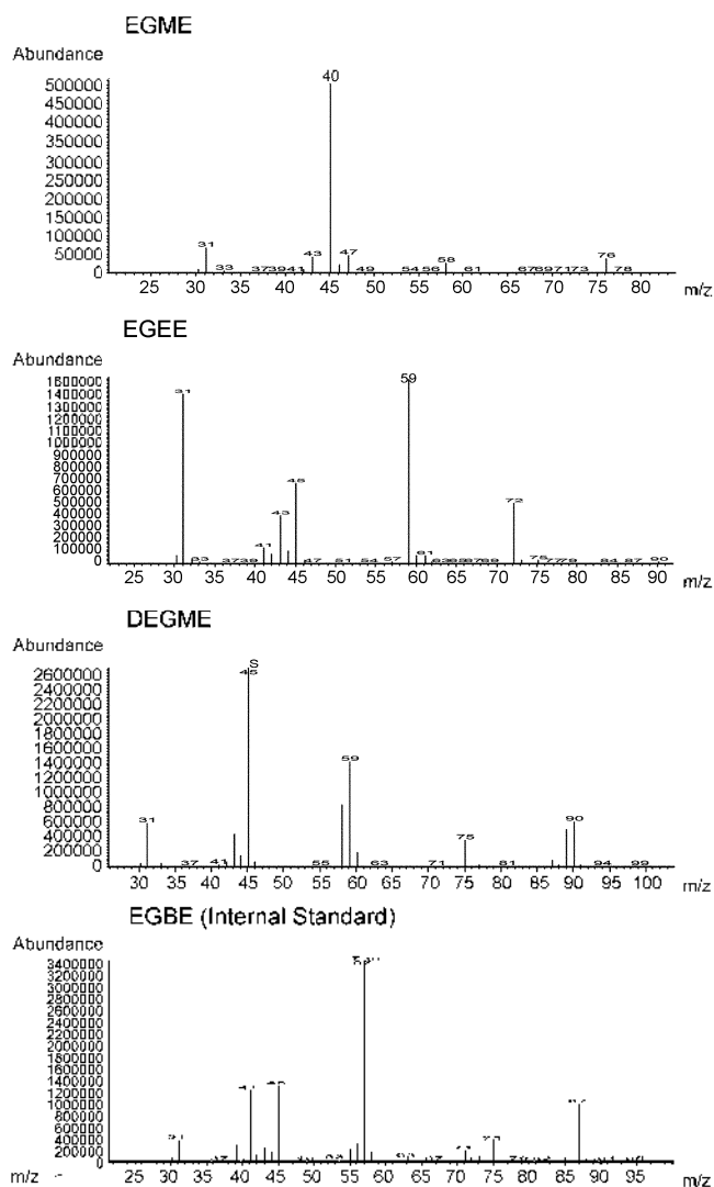
Figure 2. Mass spectra of EGME, EGEE, DEGME and EGBE.
