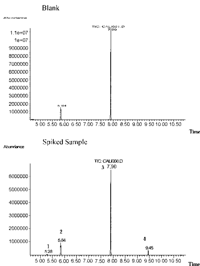
Figure 1. Chromatograms of the extracts from milli-Q water (blank) and milli-Q water spiked with 80 ng/mL of standards. (1=EGME, 2=EGEE, 3=EGBE, 4=DEGME).
