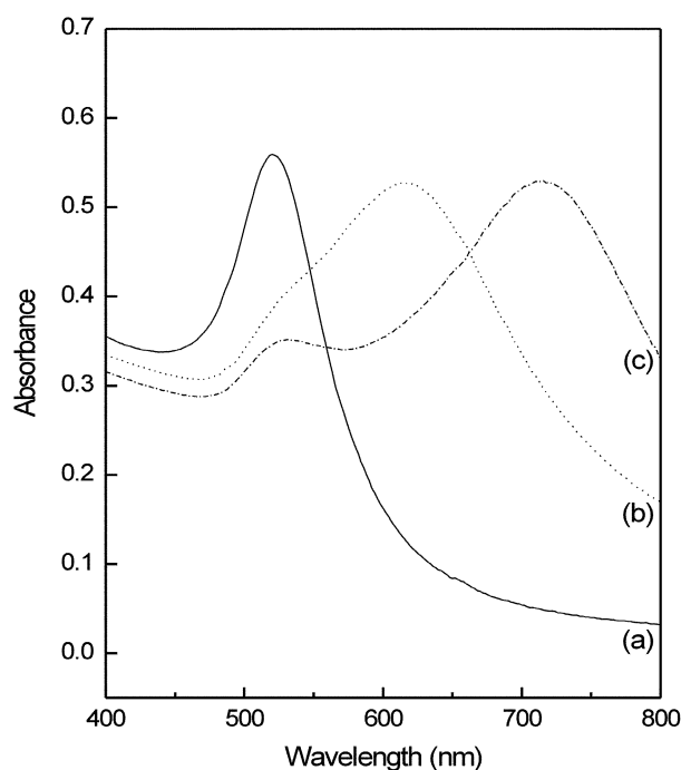
Figure 2. Plots of UV-Visible absorption spectra of gold nanoparticles: (a) in the absence of DPC (the solid line), (b) 5 minutes after modifying with 1 \times 10 -4 M DPC (dotted line), and (c) 5 \times 10 -2 M DPC (the dash-dotted line).
