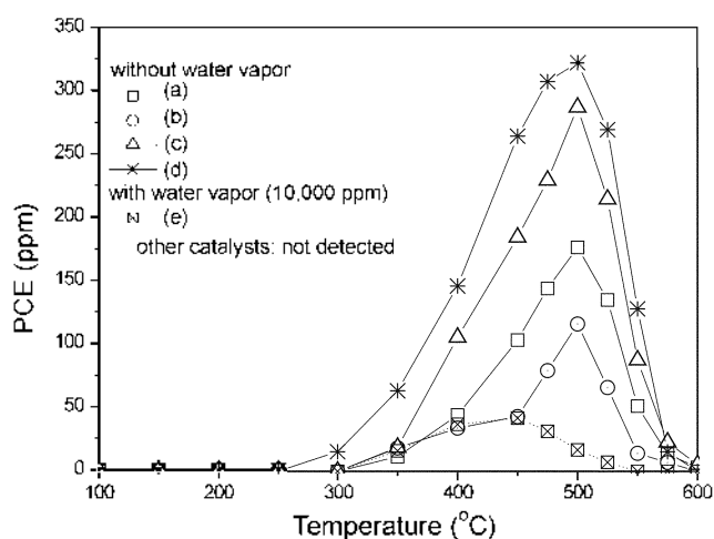
Figure 6. Concentrations of generated PCE as a function of temperature during the oxidation of TCE over various catalysts: (a) Pd(0.5)/SO 4 -ZrO 2 , (b) Pd(1.0)/SO 4 -ZrO 2 , (c) Pd(1.5)/SO 4 -ZrO 2 , (d) Pd(1.0)/ZrO 2 , (e) Pd(1.0)/ZrO 2 , other catalyst: not detected. Reaction conditions: TCE = 1.000 ppm, H 2 O = 10.000 ppm, GHSV = 14,000 h -1 .
