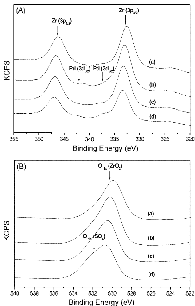
Figure 4. X-ray photoelectron (XP) spectra of (A) Zr_{3p} and Pd_{3d} , and (B) O_{1s} core levels on Pd(1.0)/ZrO_2 and Pd(1.0)/SO_4-ZrO_2 catalysts: (a) ZrO_2 , (b) Pd(1.0)/ZrO_2 , (c) SO_4-ZrO_2 and Pd(1.0)/SO_4-ZrO_2 .
