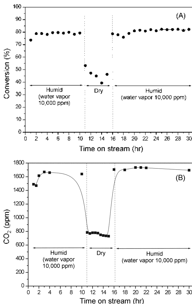
Figure 1. Effect of water vapor addition for the TCE conversion and \text{CO}_2 formation over \text{Pd}(1.0)/\text{SO}_4\text{-ZrO}_2 catalyst at 500 °C. Reaction conditions: TCE = 1,000 ppm, \text{H}_2\text{O} = 10,000 ppm, GHSV = 20,000 \text{h}^{-1} .
