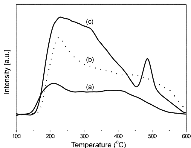
Figure 3. NH 3 -TPD profiles of (a) SO 4 -ZrO 2 , (b) Pd(1.0)/ZrO 2 , and (c) Pd(1.0)/SO 4 -ZrO 2 catalysts.
