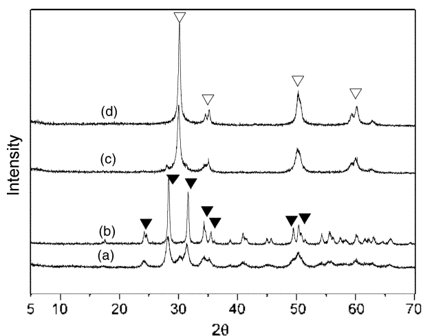
Figure 2. XRD patterns of (a) ZrO 2 , (b) Pd(1.0)/ZrO 2 , (c) SO 4 -ZrO 2 , and (d) Pd(1.0)/SO 4 -ZrO 2 catalysts, where ▼ and ▲ indicate monoclinic phase and tetragonal phase, respectively.
