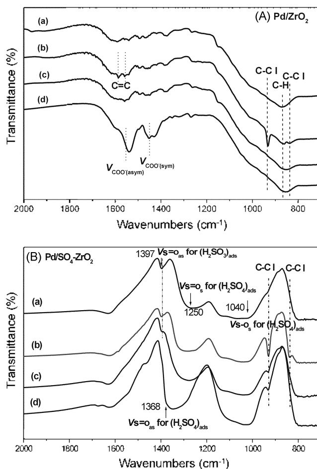
Figure 5. FT-IR spectra on adsorption/desorption of TCE over (A) Pd(1.0)/ZrO_2 and (B) Pd(1.0)/SO_4-ZrO_2 catalysts: (a) pretreatment at 350 °C for 5 hr, (b) adsorption 7 torr at RT, (c) desorption at room temperature by evacuation, and (d) desorption at 300 °C by evacuation.
