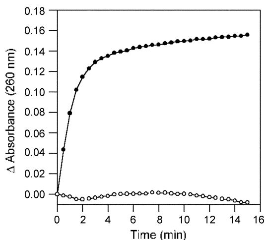
Figure 5. DNase I protection assay of PEG- b -poly(L-lysine) dendrimer/pSV- \beta -gal DNA complex. The difference in absorbance at 260 nm versus time was plotted. Plasmid DNA only ( \bullet ), and 5.6 \mu g of copolymer per 1.0 \mu g of plasmid DNA ( \circ ).
