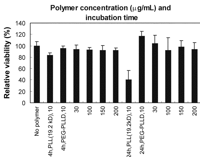
Figure 6. Effect of poly(L-lysine) and PEG-PLL ( G = 4 ) on the viability of 293 cells. Relative viability is expressed considering the absorbance at 570 nm of intact cells as 100%. Each data point is the average \pm SD of six different experiments.
