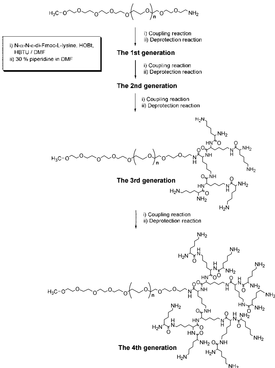
Figure 1. Outline of step-wise liquid phase synthesis of poly(ethylene glycol)- block -poly(L-lysine) dendrimer (PEG-PLL.D).
