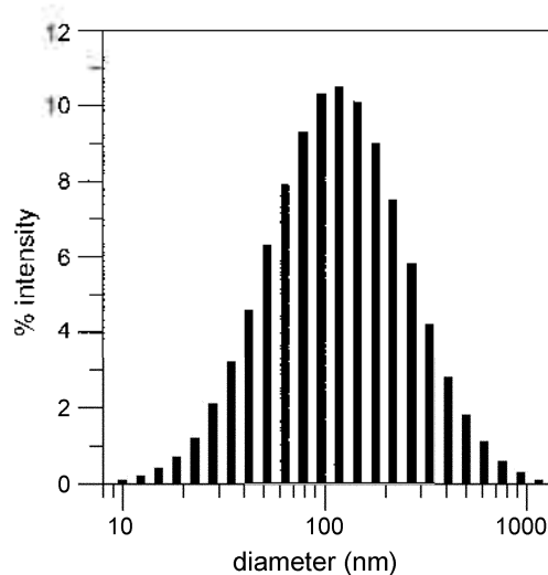
Figure 3. Dynamic light scattering of PEG-PLL D/pSV- \beta -gal plasmid DNA complexes.
