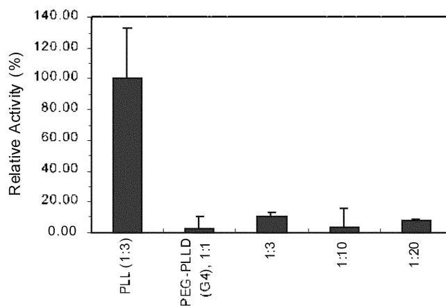
Figure 7. Transfection efficiency for 293 cell lines. The weight ratio of DNA and poly(L-lysine) was 1 \mu g and 3 \mu g per well, respectively (1 : 3). Various weight ratios of DNA : PEG-PLL ( G = 4 ) were tested as indicated.
