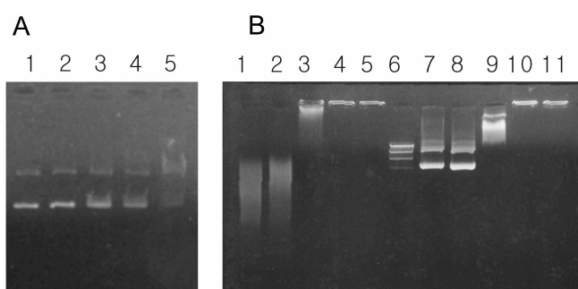
Figure 2. Analysis of complex formation at various charge ratios by agarose gel electrophoresis. (A) PEG-PLL D (generation 3) 1.0 \mu\text{g} of pSV- \beta -gal plasmid DNA only (Lane 1), charge ratio of copolymer/DNA = 0.5, 1, 2, and 4 (Lane 2, 3, 4, and 5, respectively). (B) PEG-PLL D (generation 4) 1.0 \mu\text{g} of sheared Herring testes DNA only (Lane 1), charge ratio = 0.5, 1, 2, and 4 (Lane 2, 3, 4, and 5, respectively). Lane 6 is \lambda /HindIII cut DNA marker (23.1, 9.4, 6.5, 4.3 kbp). 1.0 \mu\text{g} of pSV- \beta -gal plasmid DNA only (Lane 7), charge ratio of copolymer/DNA = 0.5, 1, 2, and 4 (Lane 8, 9, 10, and 11, respectively).
