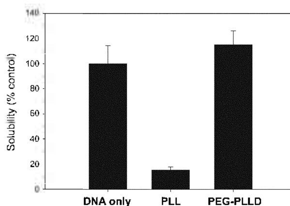
Figure 4. Water-solubility test of PEG-PLL D/DNA polyplex. Poly(L-lysine) was used as control reagent.
