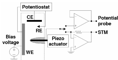
Figure 1. Schematic presentation of the apparatus. In an electrochemical cell depicted by the broken-lined box, a potential probe approaches the WE surface and monitors the local potential of the electrochemical interface. The voltage follower accessed by switching from the STM mode reads the potential without passing tunneling currents.
