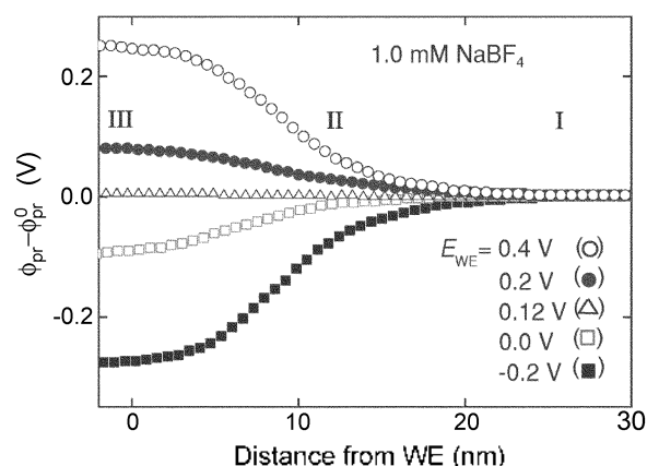
Figure 2. The potential measured at the probe as it approaches the Au(111) surface of the WE immersed in a 1.0 mM \text{NaBF}_4 solution. The distance to the bulk is measured from the point of a mechanical contact between the probe and the electrode surface.
