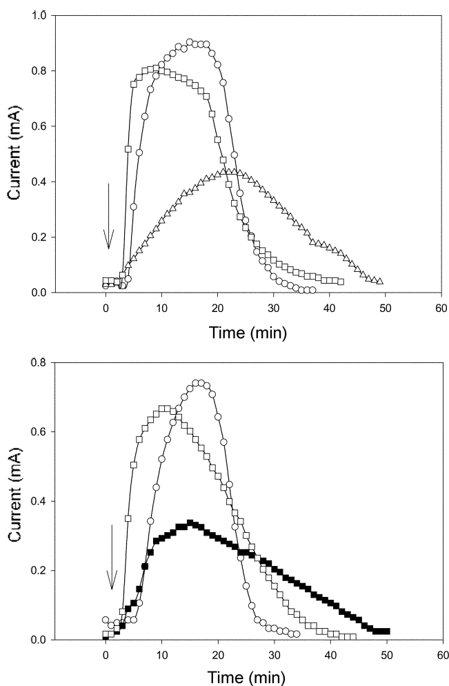
Figure 4. Variation of current outputs with time for bacterial fuel cells containing (A) B. licheniformis and (B) B. thermoglucosidasius (organism concentration: 1 mg (dry wt) mL -1 ; 4.0 \mu mol of azure A and 1.0 \mu mol of 11 different utilized carbon sources such as fructose, galactose, glucose, lactose, maltose, mannitol, mannose, sorbitol, starch, sucrose and trehalose; external resistive load: 300- \Omega ). Measurable current outputs were detected only four utilized carbon sources, glucose ( \square ), maltose ( \blacktriangle ), mannose ( \blacksquare ), and trehalose ( \square ). Thermophilic microorganisms were initially grown in yeast extract, a complex medium before the fuel cell operation.
