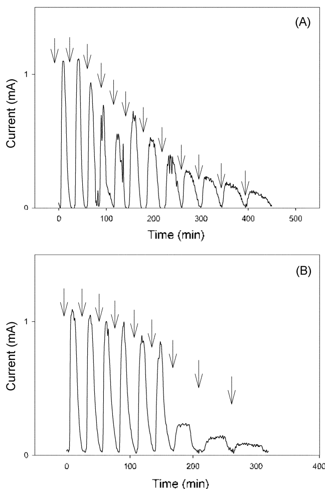
Figure 5. Variation of current output with time through the 300 \Omega external load for bacterial fuel cells containing B. thermoglucosidasius (1 mg (dry wt) mL -1 ) and the repetitive addition 1.0 \mu mol of carbon source in the presence of azure A (4 \mu mol); initial carbon source for bacterial culture: (A) lactose (B) mannitol, utilized carbon source for fuel cell operation: (A) glucose (B) mannitol. The constant amount of a carbon source was added after the current output reached a background level.
