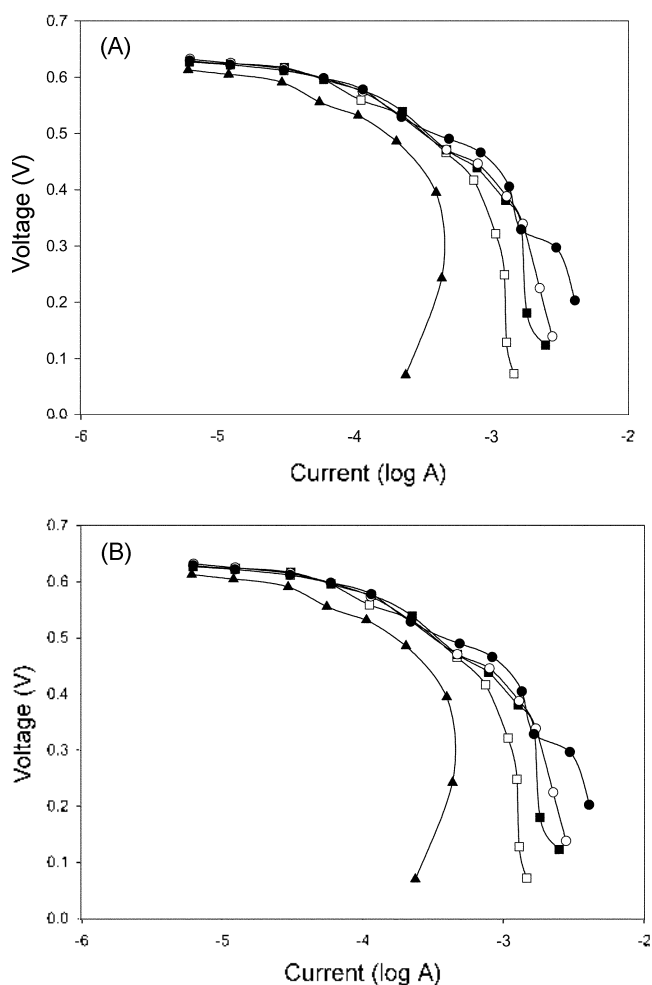
Figure 2. Current-voltage curves for fuel cells containing (A) B. licheniformis (B) B. thermoglucosidasius obtained at 30 °C (□), 40 °C (■), 50 °C (○), 60 °C (●), and 70 °C (▲) with azure A as a mediator. Organism concentration: 2 mg (dry wt) mL -1 ; 4 μmol of mediator and 100 μmol of glucose added initially.
