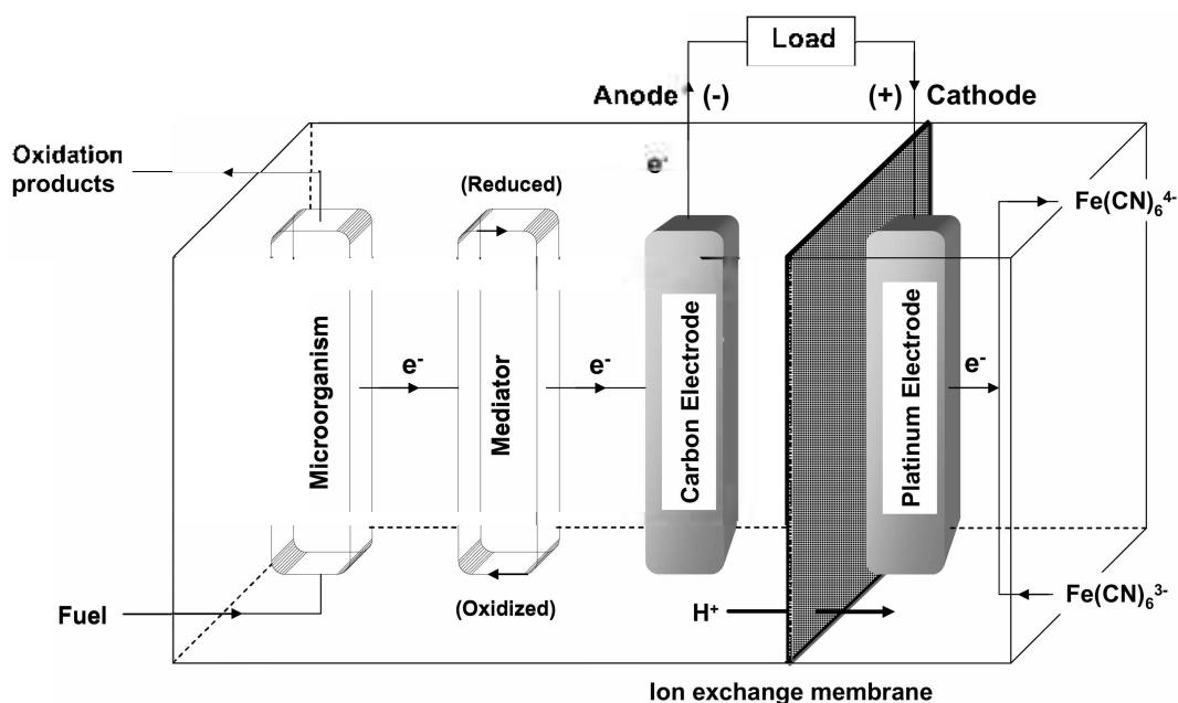
Figure 1. Schematic diagram showing the principal features of a microbial fuel cell.
