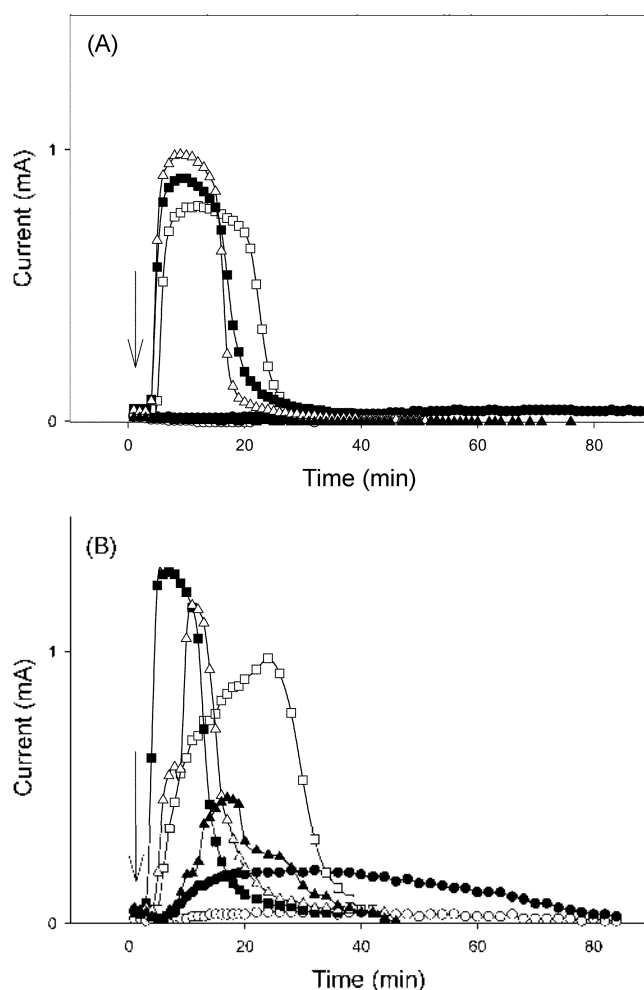
Figure 3. Variation of current output with time through the 300-Ω external load for fuel cells containing (A) B. licheniformis (B) B. thermoglucosidasius obtained at different buffer pH 5 (○), 6 (●), 7 (□), 8 (■), 9 (▲), and 10 (▲) on the addition 1.0 μmol of glucose. Organism concentration: 1 mg (dry wt) mL -1 ; azure A: 4 μmol.
