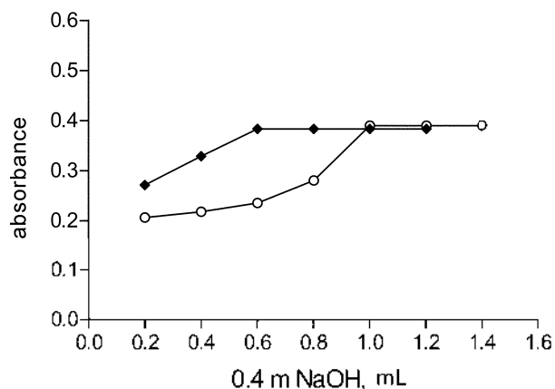
Figure 5. Effect of \text{NaOH} ◆ Carbocisteine; ○ Penicillamine ( 10 \mu\text{g}/\text{mL} of each drug).
