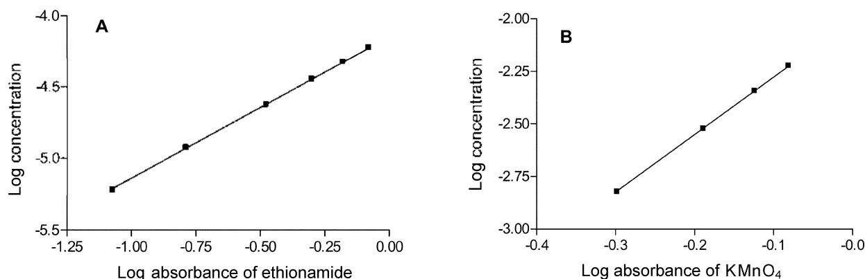
Figure 10. Stoichiometry of the reaction between Ethionamide and \text{KMnO}_4 adopting limiting logarithmic method A: Ethionamide B: \text{KMnO}_4 .
