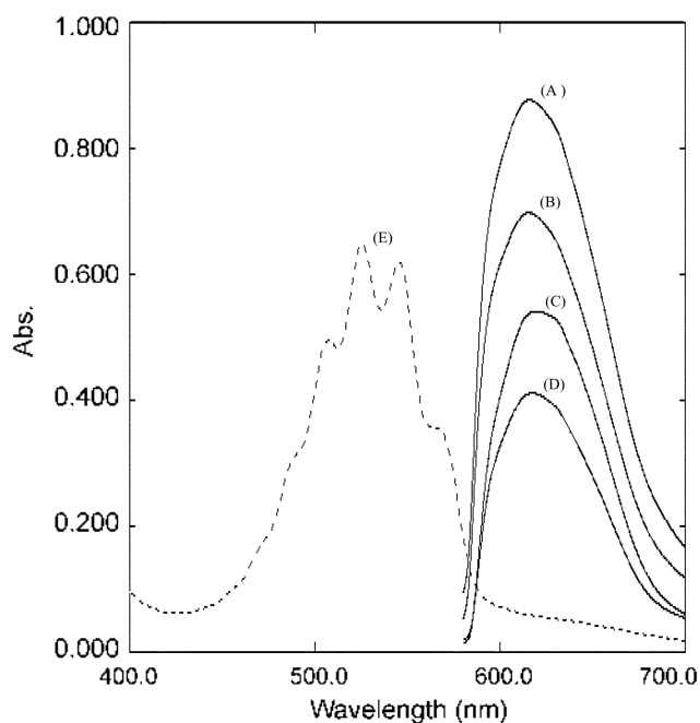
Figure 1. Absorption spectra of the reaction product with \text{KMnO}_4/\text{NaOH} system: (A) Reaction product of ethionamide ( 10 \mu\text{g}/\text{mL} ), (B) Reaction product of thioctic acid ( 10 \mu\text{g}/\text{mL} ), (C) Reaction product of carbocisteine ( 10 \mu\text{g}/\text{mL} ), (D) Reaction product of penicillamine ( 10 \mu\text{g}/\text{mL} ), (E) \text{KMnO}_4 ( 1.97 \times 10^{-1} \text{ M} ).
