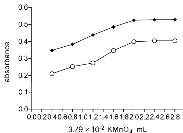
Figure 3. Effect of \text{KMnO}_4 ◆ Carbocisteine; ○ Penicillamine ( 10 \mu\text{g}/\text{mL} of each drug).
