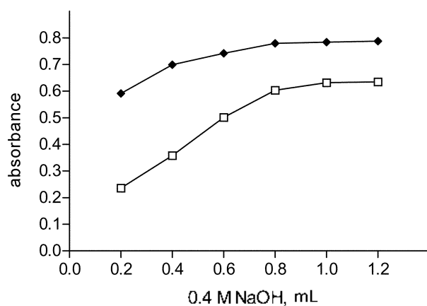
Figure 4. Effect of \text{NaOH} ◆ Ethionamide; □ Thioctic acid ( 10 \mu\text{g}/\text{mL} of each drug).
