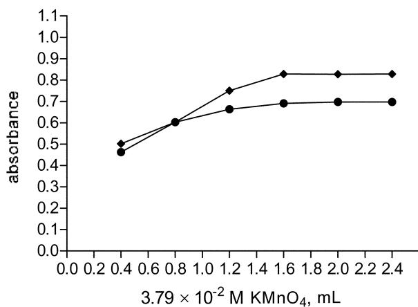
Figure 2. Effect of \text{KMnO}_4 ● Thioctic acid; ◆ Ethionamide ( 10 \mu\text{g}/\text{mL} of each drug).
