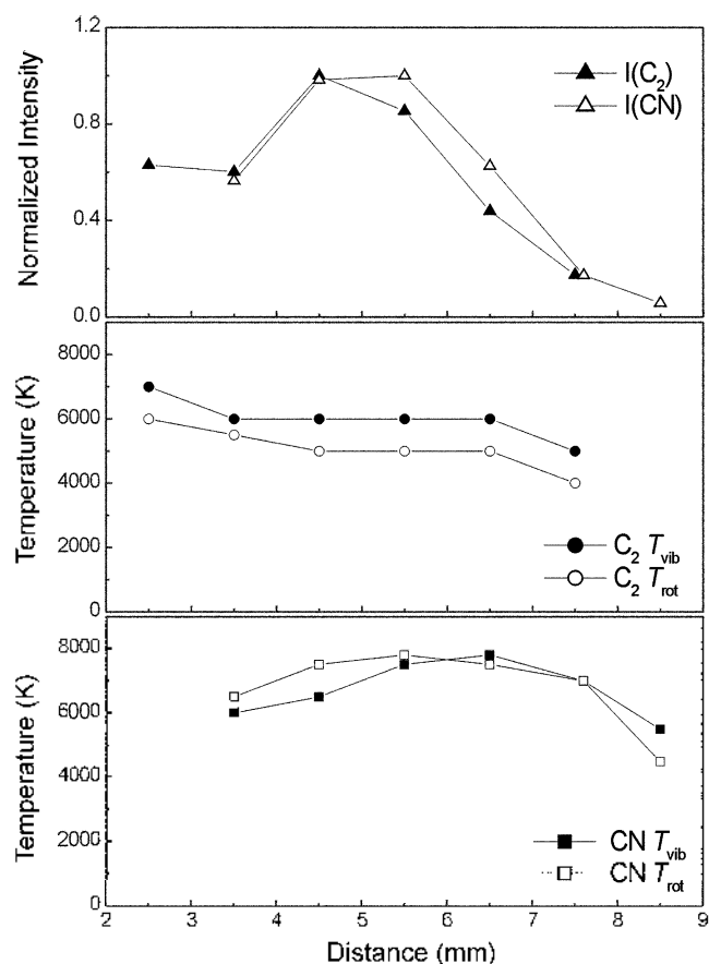
Figure 6. The normalized emission intensities, I(C_2) and I(CN) , vibrational ( T_{vib} ) and rotational ( T_{rot} ) temperatures determined from the optical emission spectra of C_2 and CN molecules as a function of the distance from the target. The laser fluence was 2.7 \text{ J/cm}^2 and the pressure of N_2 was 10 Torr.
