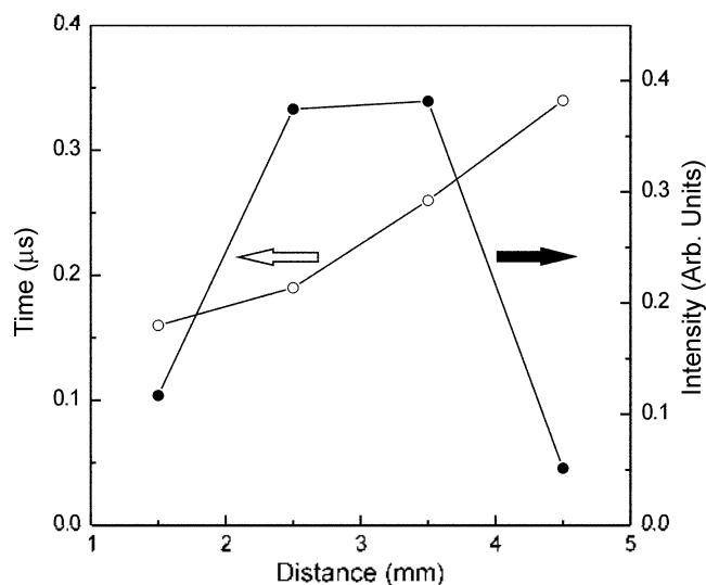
Figure 7. The emission intensity and peak arrival time of the C^+ ( 426.7 \text{ nm} ) ions as a function of the distance from the target. The laser fluence was 2.7 \text{ J/cm}^2 and the pressure of N_2 was 10 Torr.
