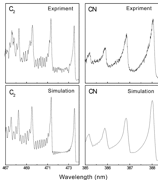
Figure 4. Comparison between the experimental and simulated spectra of C_2 ( d^1\Pi_g \rightarrow a^1\Pi_u , \Delta v = 1 ) and CN ( B^2\Sigma^- \rightarrow X^2\Sigma^+ , \Delta v = 0 ) molecules. The laser fluence was 2.7 \text{ J/cm}^2 and the pressure of N_2 was 10 Torr. The distance from the target was 4.5 mm.
