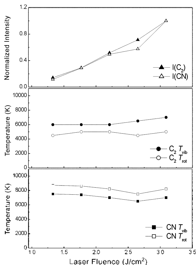
Figure 5. The normalized emission intensities, I(C_2) and I(CN) , vibrational ( T_{\text{vib}} ) and rotational ( T_{\text{rot}} ) temperatures determined from the optical emission spectra of C_2 and CN molecules at different laser fluences. The pressure of N_2 was 10 Torr and the distance from the target was 4.5 mm.
