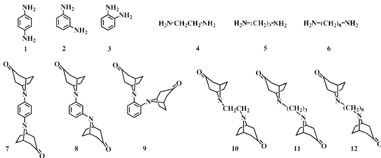
Figure 1. Structure of Di-( N -tropinonyl)benzenes and Di-( N -tropinonyl)alkanes.
