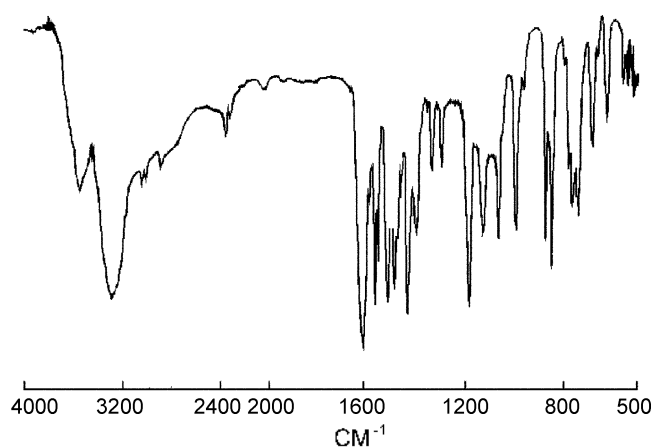
Figure 1. The infrared spectrum of QADMAA.
