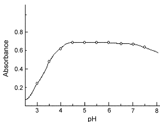
Figure 6. Effect of pH on the formation of Ni(II) complex. Ni(II) concentration was 5.0 \times 10^{-6} mol/L, other conditions as general procedure.
