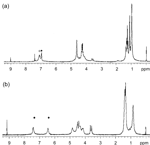
Figure 5. Proton spectra taken at the mixing ratio of (a) Calix[6] : Cs = 4 : 1 at 25 °C and (b) Calix[6] : Cs = 1 : 1 at -60 °C both in CDCl_3 . Phenyl ring proton of complexed calixarene is marked by • and those of free calixarene by ○.
