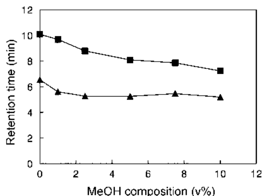
Figure 7. Variation of retention time for (▲) ammonia and (■) DCAD with MeOH composition in mobile phase of 0.02 M phosphate buffer at pH 7 on C_{18} stationary phase. Conditions: DCAD concentration 0.1 mM; KOH, 0.05 M; reaction coil, 5 m; OPA, 15 mM; reaction coil, 0.5 m; sulfite, 15 mM; coil, 6 m; 0.1 M phosphate buffer (pH 11.5); temperature 70 °C; flow rate, 0.5 mL/min; 100 \mu L injection; fluorescence detector, \lambda_{ex} = 363 nm, \lambda_{em} = 425 nm.
