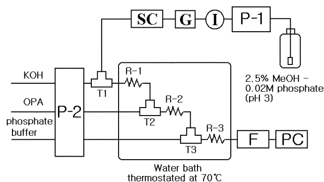
Figure 1. Schematic diagram of RPLC-postcolumn detection for determination of DCAD. P-1: high pressure pump, I: injector (100 μL); G: guard column; SC: Nova-Pak C 18 separation column; P-2: peristaltic pump; T: mixing tee; R: reaction coil; F: fluorescence detector. λ ex 363 nm, λ em 425 nm.
