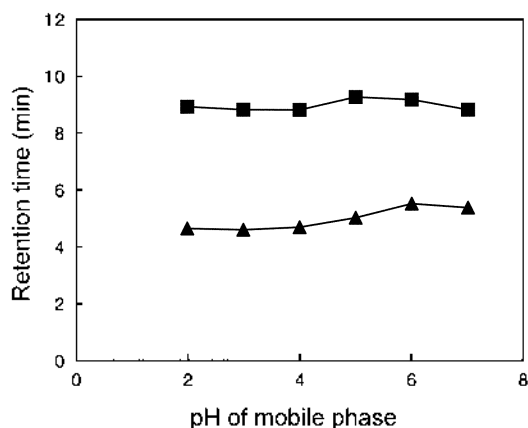
Figure 8. Variation of retention time for (▲) ammonia and (■) DCAD with pH in mobile phase of 2.5% MeOH-0.02 M phosphate buffer on C_{18} stationary phase. The optimal conditions for postcolumn derivatization were the same as in Figure 7.
