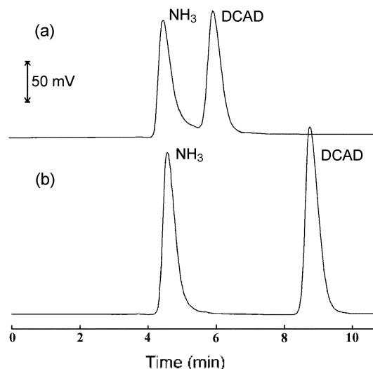
Figure 9. Liquid chromatogram of ammonia and DCAD mixture by RPLC-postcolumn derivatization. Conditions: column, Nova-Pak C_{18} (3.9 \times 150 mm); (a) 10%MeOH-0.02 M phosphate buffer (pH 7), 0.05 M ammonia, 0.05 mM DCAD (b) 2.5%MeOH-0.02 M phosphate buffer (pH 3), 0.1 mM ammonia, 0.1 mM DCAD; flowrate, 0.5 mL/min; 100 \mu L injection; Fluorescence detector, \lambda_{ex} = 363 nm, \lambda_{em} = 425 nm. Other postcolumn detection conditions were the same as Figure 6.
