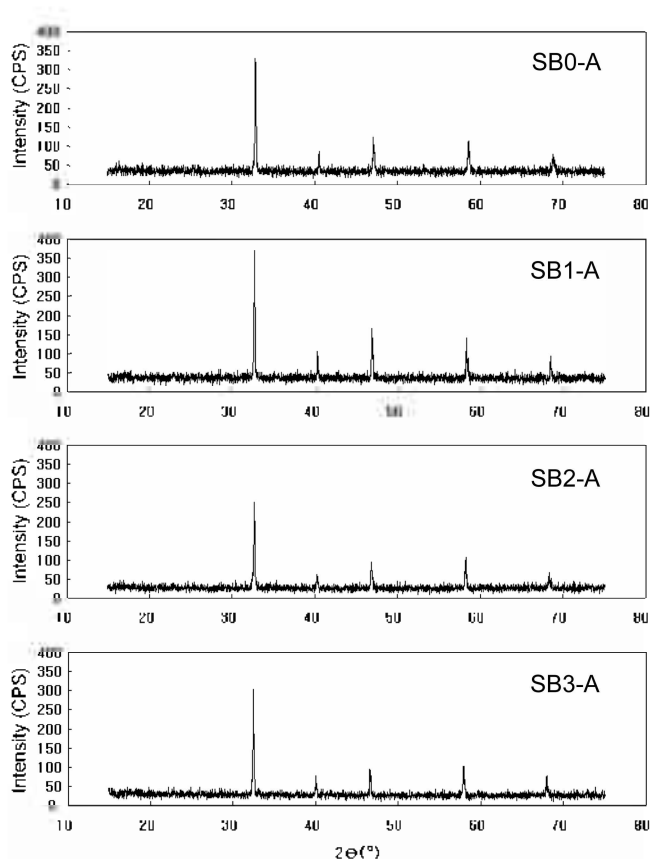
Figure 1. X-ray powder diffractograms of SB0-A, SB1-A, SB2-A and SB3-A samples of Sr_{1-x}Ba_xFe^{3+}_{1-\tau}Fe^{4+}_{\tau}O_{3-y} system.
