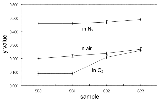
Figure 3. Variations of y values of the \text{Sr}_{1-x}\text{Ba}_x\text{Fe}^{3+}_{1-7}\text{Fe}^{4+}_7\text{O}_{3-y} samples.
