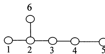
Figure 1. Labeled hydrogen depleted graph of 2-methylpentane.
