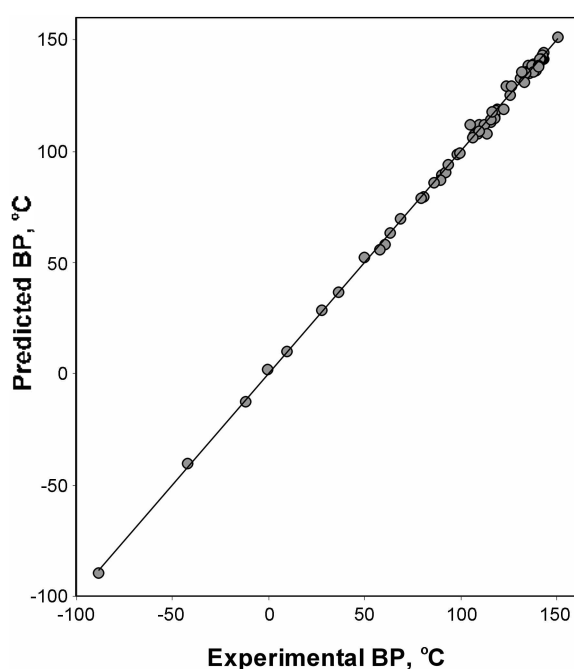
Figure 3. Plot of predicted boiling point of alkanes C_2-C_9 (using MLR) versus experimental boiling points.
