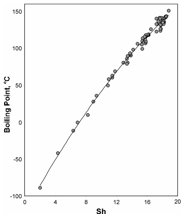
Figure 2. Plot of boiling points of C 2 -C 9 alkanes versus Sh index.
